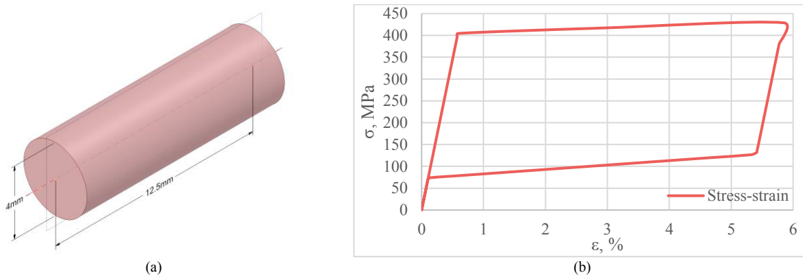
Fig.3 NiTi sample model (a) and hysteresis loop (b).
