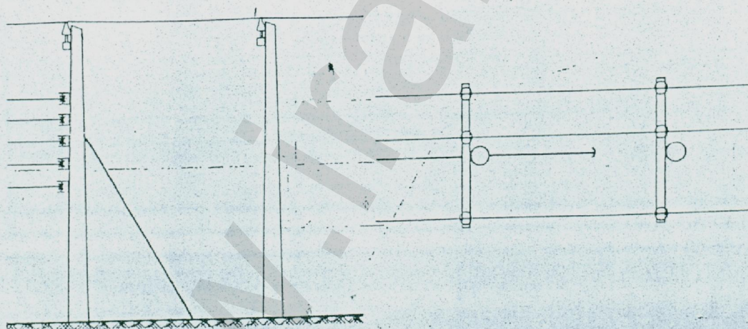
SECONDARY DEAD END THROUGH PRIMARY
