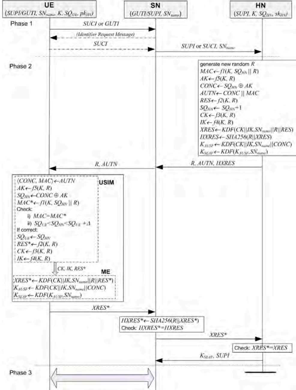
Fig. 2. 5G-authentication and key agreement (AKA).
