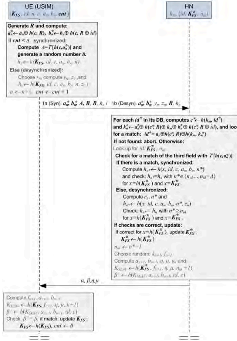
Fig. 4. The enhanced Braeken AKA protocol with forward-security.
