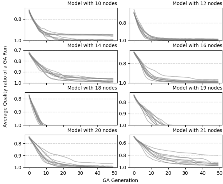
Figure 8: Convergence rate of 10 GA runs per model
