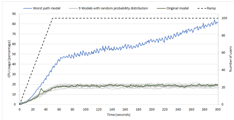
Figure 6: CPU utilization created by the models
