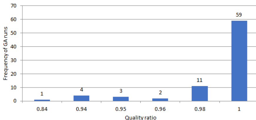
Figure 9: Frequency distribution of all GA runs based on the quality ratio
