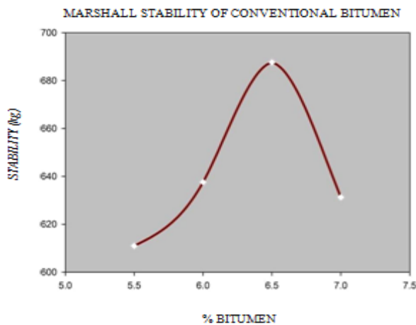
Fig. 10: variation of marshall stability for proposed bituminous mixes
