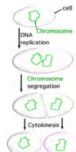
Binary Fission
