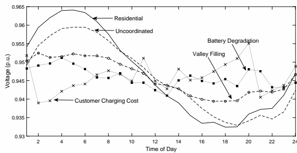
Fig. 8. Voltage profile of Node 844 under different schemes
