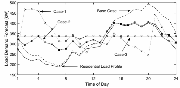
Fig. 5. Optimal load demand forecast under individual objectives
