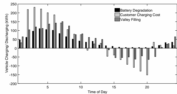
Fig. 9. Optimal EV charging/discharging profiles under individual objectives
