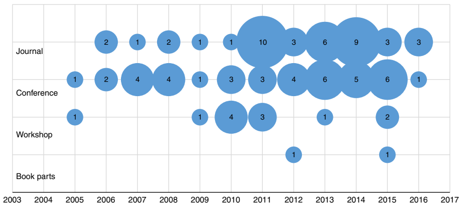
Figure 4. Primary studies publication per year
