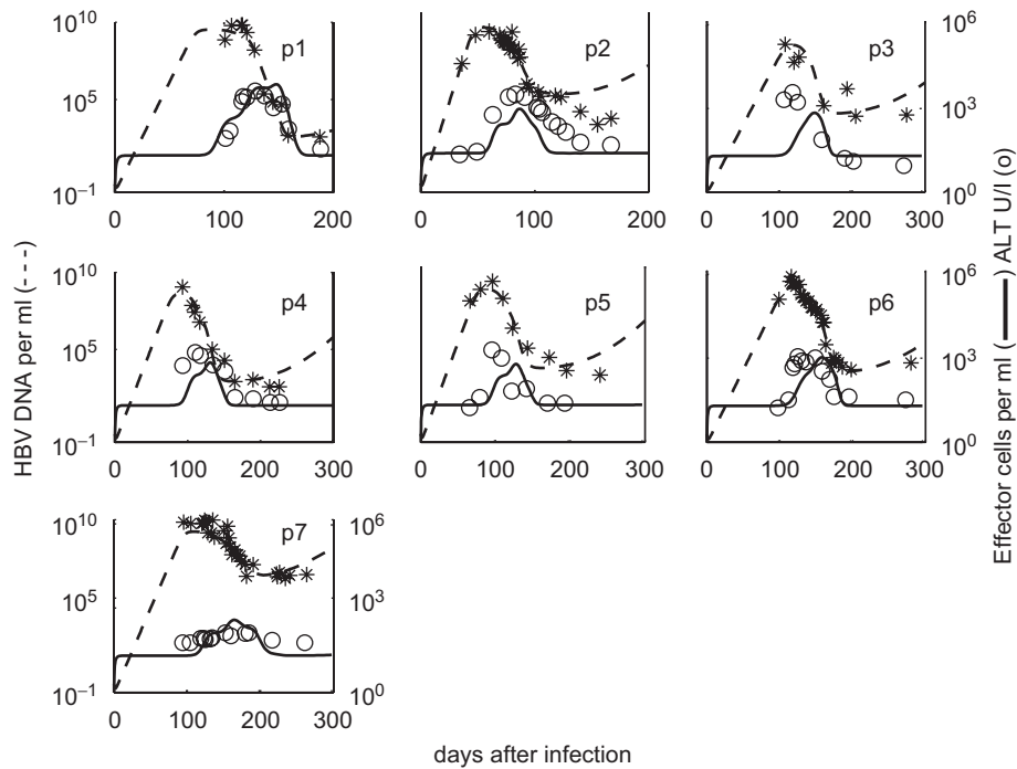
Fig. 7. Results of fitting the model with one class of infected cells to the data. The best fit of the model (dashed line) to HBV DNA patient data (*). The measured serum ALT ( \circ ), which was not used in data fitting, compares well with the predicted dynamics of the HBV-specific CD8^+ T-cell response (solid line).
