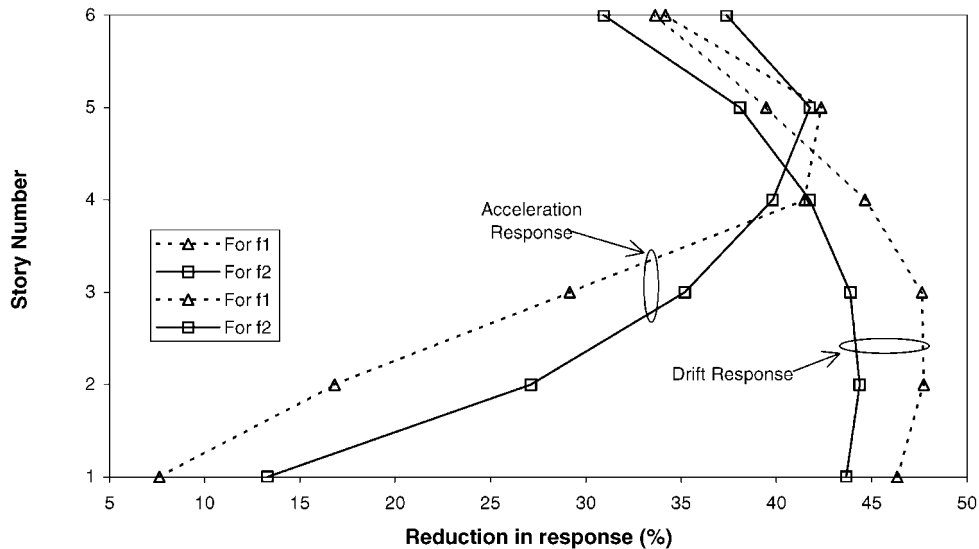
Figure 6. Percent reduction in story drifts and floor accelerations in X -direction for tuned mass dampers designed for f_1 (Equation (3)) and f_2 (Equation (4)) performance functions; Kanai-Tajimi PSDF input.
