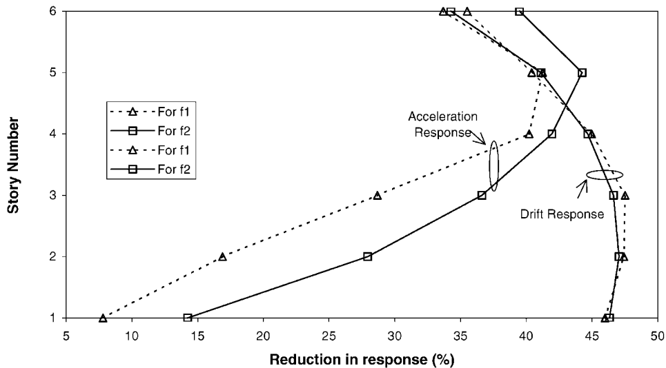
Figure 7. Percent reduction in story drifts and floor accelerations in Y -direction for tuned mass dampers designed for f_1 (Equation (3)) and f_2 (Equation (4)) performance functions; Kanai-Tajimi PSDF input.
