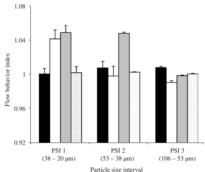
Fig. 4. Flow behavior index of chocolate samples manufactured with sucrose (■), isomalt (□), xylitol (▒), and maltitol (▨) in different particle size intervals (PSI). Error bars represent standard deviations.
