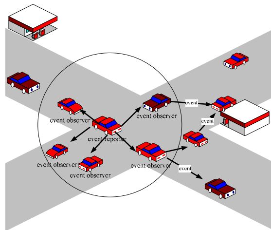
Figure 1. Categorize Member
