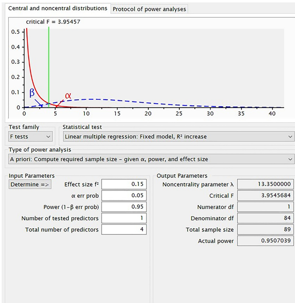
Figure 2. Power results for required sample size.
