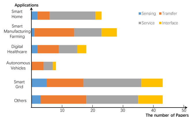
Fig. 6. The Number of Papers of Each Layer in Different IoT Application Scenarios
