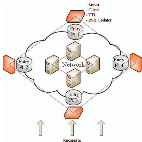
Figure 1. DSN on a network
