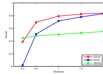
FIGURE 5. Recall on field modification replacement test case.
