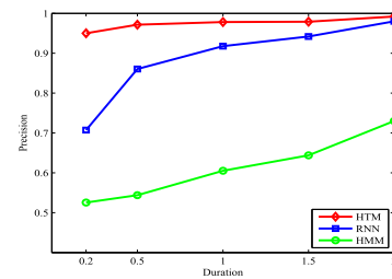
FIGURE 7. Precision on replay field replacement test case.
