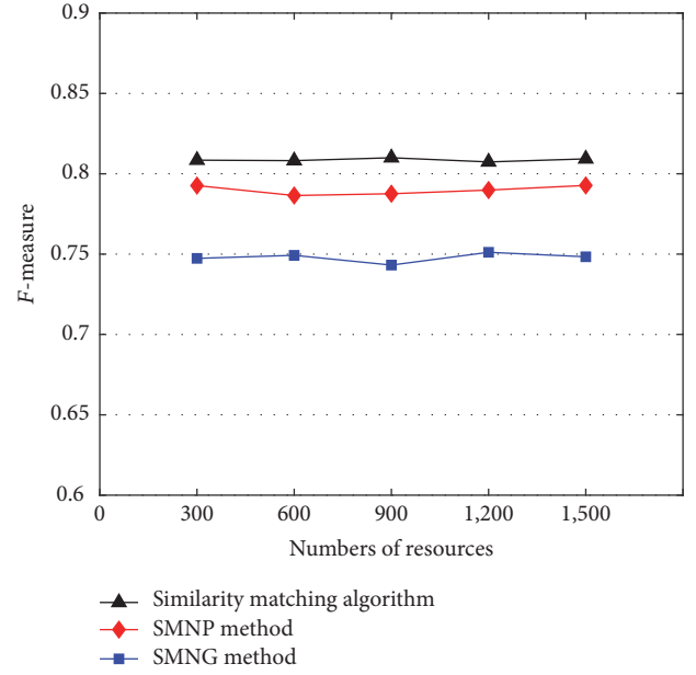
FIGURE 8: The comparison of F -measure of different methods under different numbers of resources.
