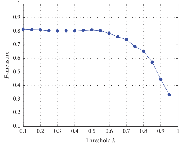
FIGURE 5: Variation of F -measure under different matching threshold.
