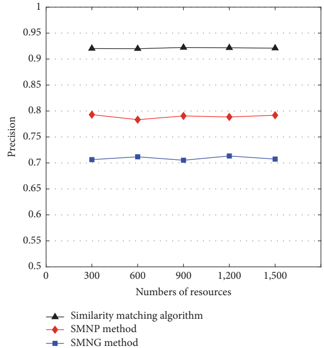
FIGURE 6: The comparison of precision of different methods under different numbers of resources.
