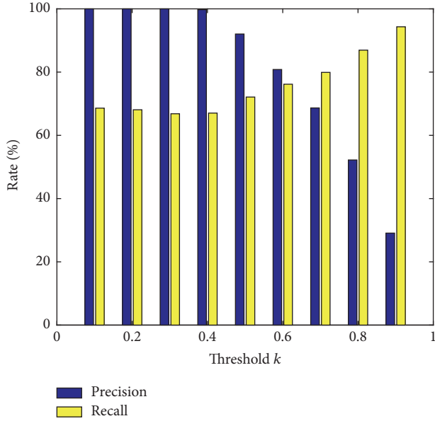
FIGURE 4: Variation of precision and recall under different matching threshold.
