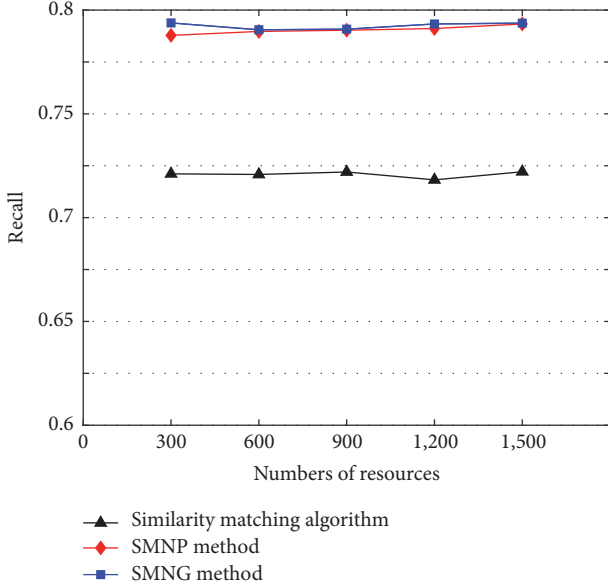
FIGURE 7: The comparison of recall of different methods under different numbers of resources.
