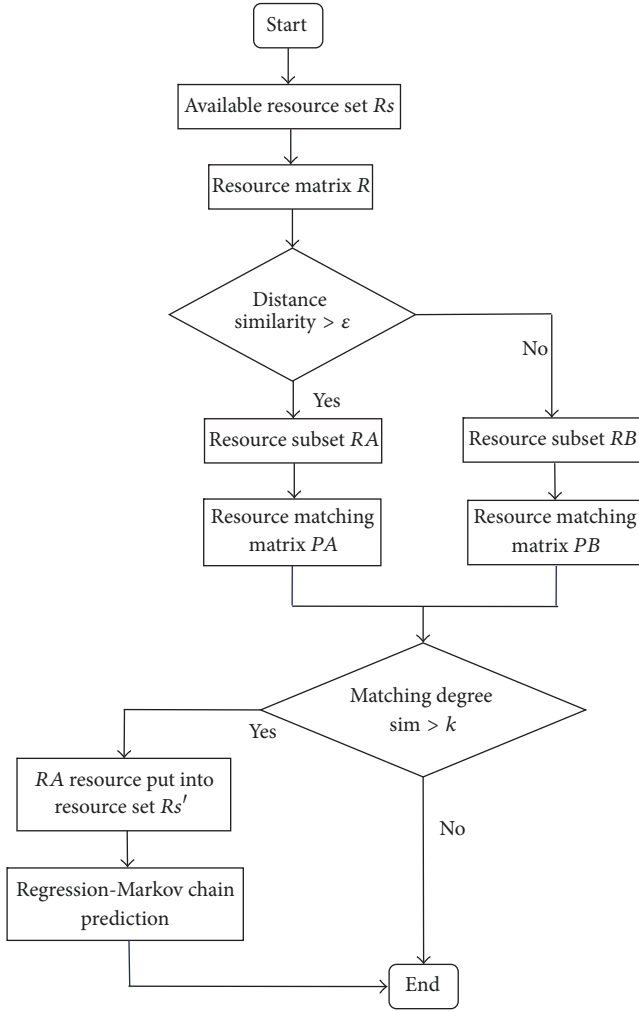
FIGURE 3: Flow chart of resource estimation method.
