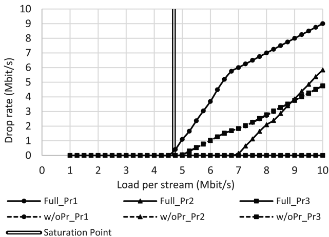
Fig. 4 Drop rate versus load per stream considering full optimisation (full) and without prioritisation (w/oPr) allocation for different traffic priorities
