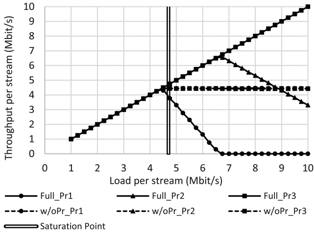
Fig. 2 Throughput versus load per stream considering full optimisation (full) and without prioritisation (w/oPr) allocation for different traffic priorities
