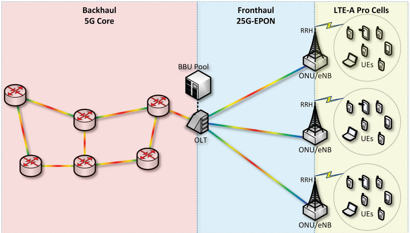
Fig. 1 Hybrid 25G-EPON and LTE-Advanced Pro FiWi architecture
