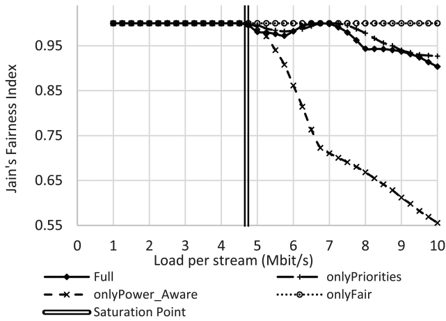
Fig. 6 Jain's fairness index versus load per stream considering full optimisation (full), only priorities (onlyPriorities), only power efficiency (onlyPower_Aware), and only fairness (onlyFair) allocation
