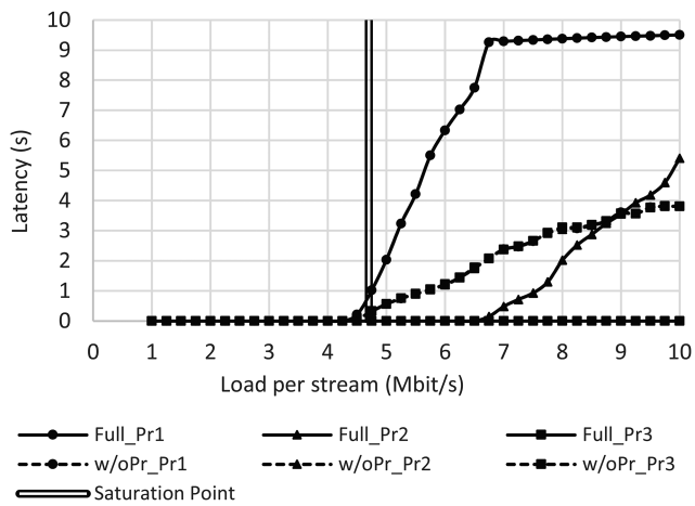
Fig. 3 Latency versus load per stream considering full optimisation (full) and without prioritisation (w/oPr) allocation for different traffic priorities
