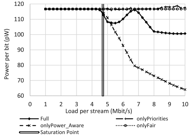
Fig. 5 Consumed power per transmitted bit versus load per stream considering full optimisation (full), only priorities (onlyPriorities), only power efficiency (onlyPower_Aware), and only fairness (onlyFair) allocation
