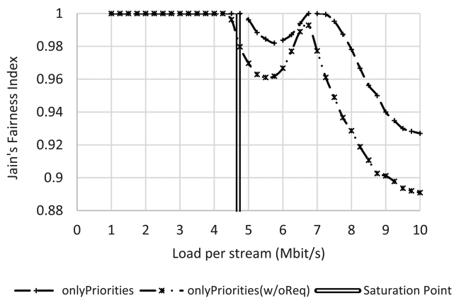
Fig. 7 Jain's fairness index versus load per stream considering only priorities including requests (onlyPriorities), and only priorities without considering requests (onlyPriorities(w/oReq)) allocation
