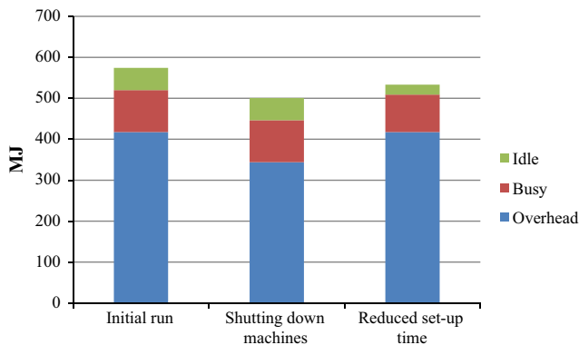
Fig. 10. Energy consumption for manufacturing one brake-set at the brake manufacturing company.
