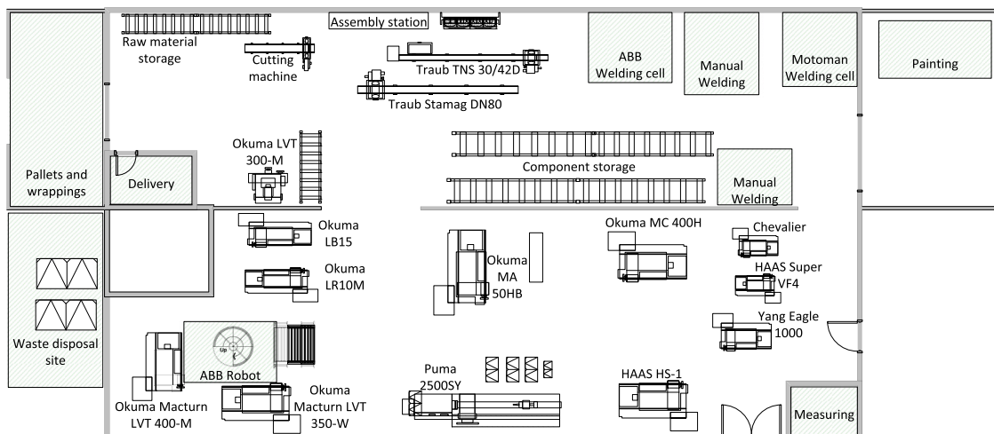
Fig. 9. Layout of the brake manufacturing factory.
