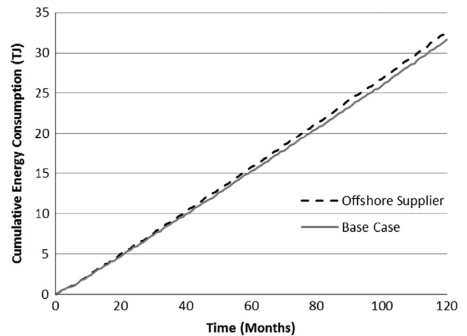
Fig. 6. Comparison of cumulative energy consumption of alternate supply chain configurations using the SD model (in Terajoules (TJ)).
