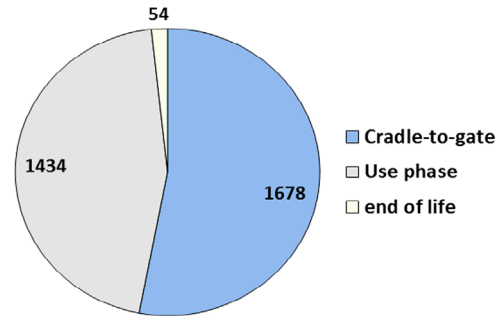
Fig. 5. Contribution of different life cycle phases to the annual energy consumption in Gigajoules (GJ).
