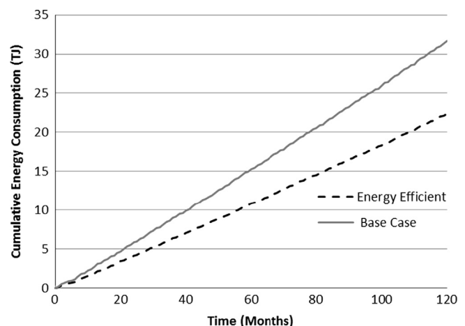
Fig. 7. Comparison of cumulative energy consumption across supply chain life cycle of base case and energy efficient scenarios using the SD model (in TeraJoules).
