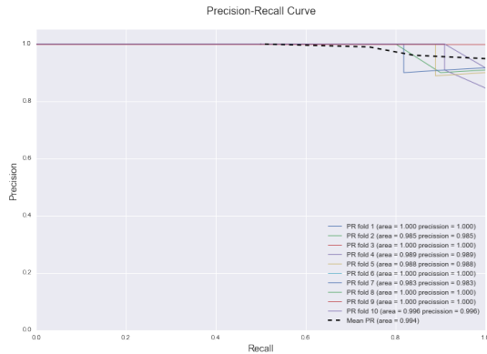
Figure 4: Precision-recall curve
