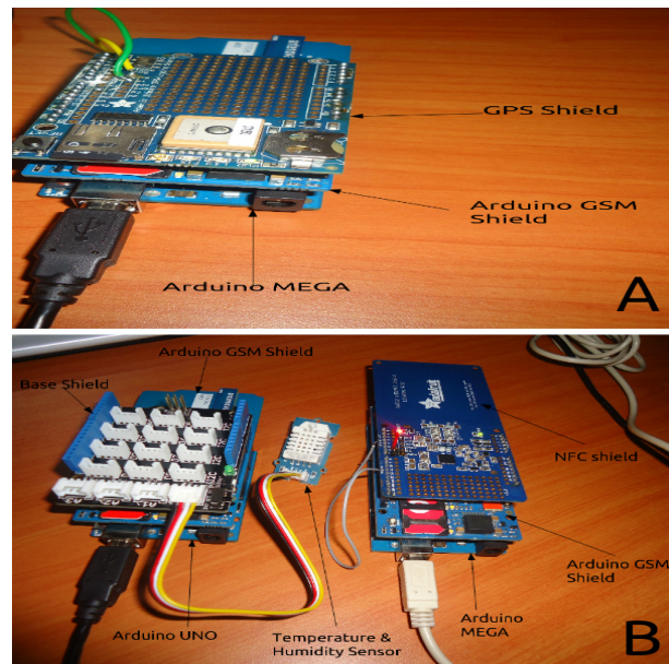
Fig. 7. Testbed
