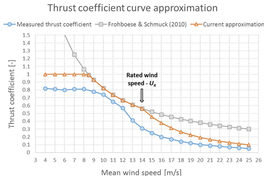
Fig. 7. Measured [41] and approximate thrust coefficients of the Vestas V80 turbine at Horns Rev.
