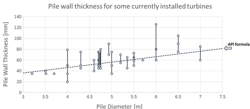
Fig. 4. Wall thickness of several currently installed wind turbines. The case studies used for the plot are collated in Appendix 1.
