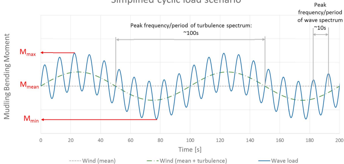
Fig. 5. Mudline moment due to wind and wave load, wind and waves collinear.
