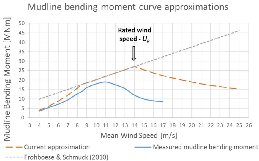
Fig. 6. Measured and approximated mudline bending moments of Horns Rev offshore wind turbine. The measured data is obtained from Hald et al. [41].
