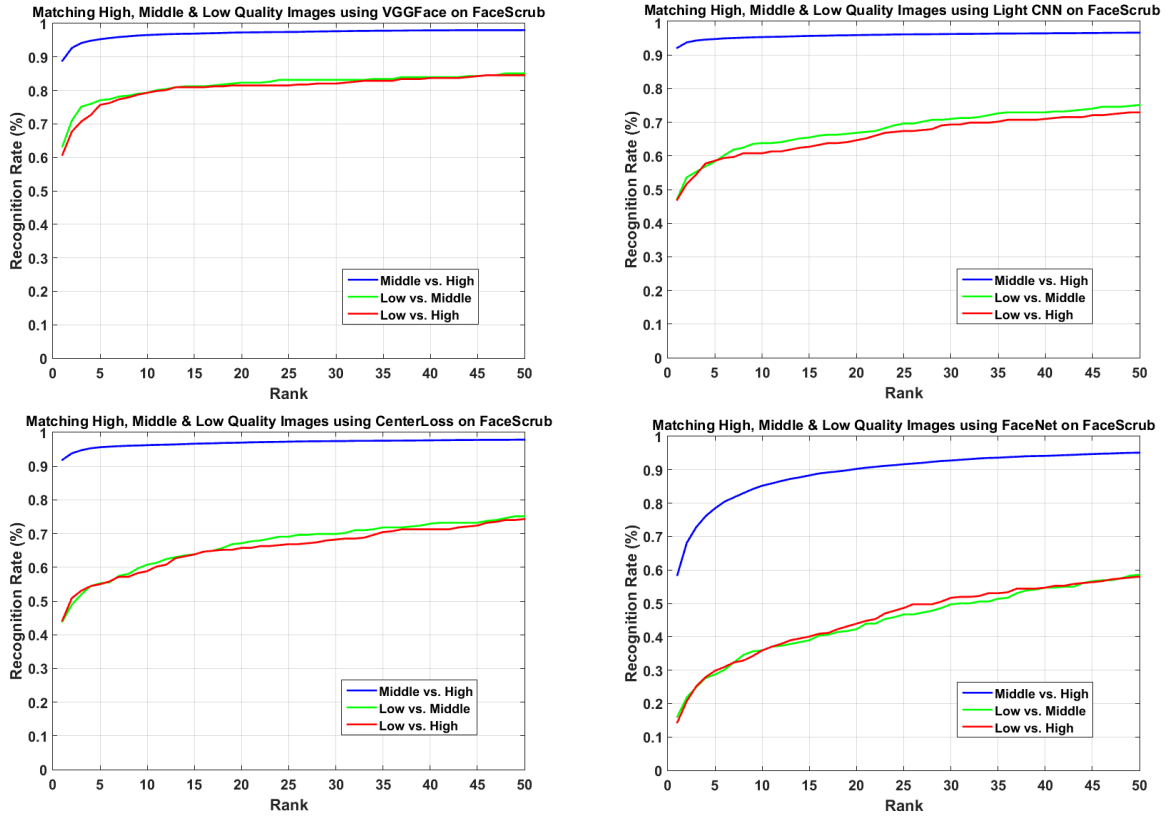
Fig. 3. Face identification across quality changes on the FaceScrub database: Top Left: VGGFace, Top Right: Light CNN, Bottom Left: CenterLoss, and Bottom Right: FaceNet. The matching is performed in three cases for each model: Middle vs. High, Low vs. Middle, and Low vs. High.
