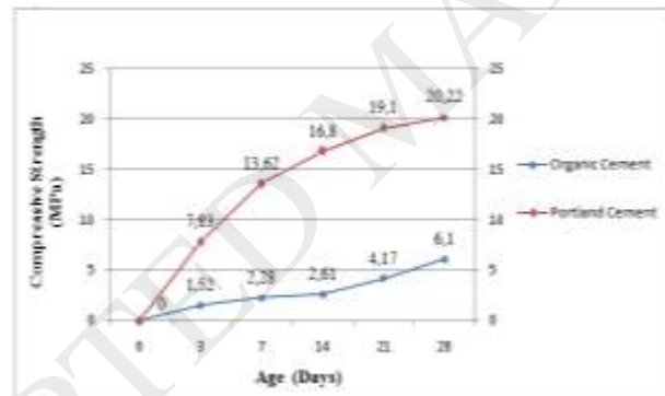
Figure 3. Graph compressive strength of organic and portland cements
