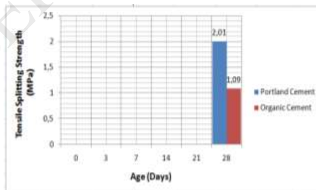
Figure 4. Graph of tensile splitting strength with water curing method
