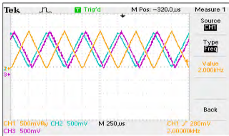
Fig. 21. PWM carrier for each LC. (Orange: converter1; Cyan: converter 2; Magenta: converter 3). (For interpretation of the references to color in this figure legend, the reader is referred to the web version of this article.)
