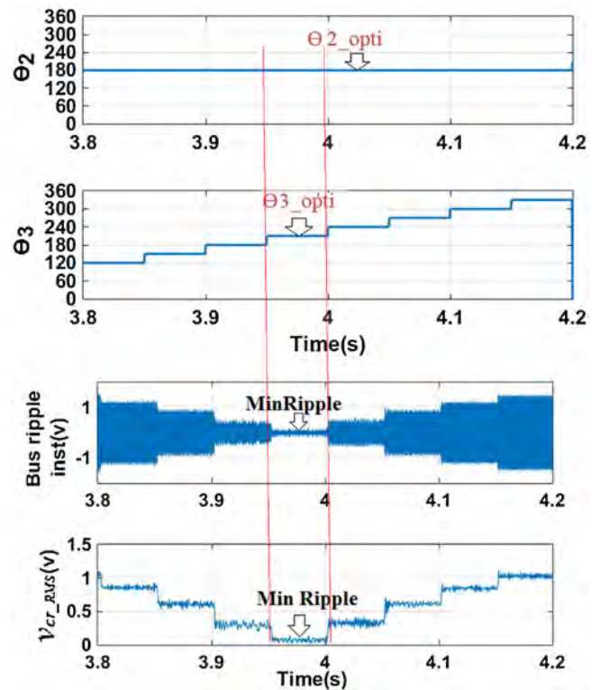
Fig. 13. Minimum ripple and optimum phase shift detection.
