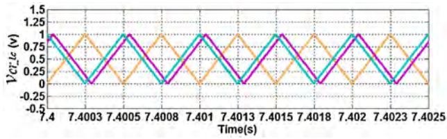
Fig. 14. PWM carriers based on optimum phase shift angles. (Orange: converter 1; Cyan: converter 2; Magenta: converter 3). (For interpretation of the references to color in this figure legend, the reader is referred to the web version of this article.)
