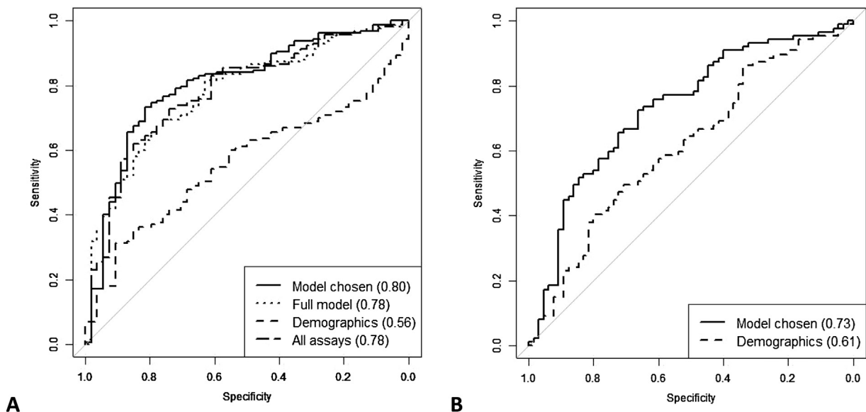
Fig. 1. A. Receiver operating characteristic (ROC) curves to predict the probability of epilepsy (combined focal and generalised) compared to control subjects. Four different models are presented: the stepwise selected model (model chosen); the full model with all the variables; the model with only age and gender (demographics); and the model with only the eleven complement assays. The most accurate model is the stepwise selected model (AUC = 0.80), followed by the full model and the model including the eleven assays only (AUC = 0.78). The model with only the demographics provides poor performance (AUC = 0.56). B. ROC curves for controlled versus uncontrolled cases: Two models are presented, the selected model (age alongside iC3b, C3, C4, Properdin, CRP) and the model with only the demographics variables. The selected model is significantly more accurate (AUC = 0.73) than the model with demographics alone (AUC = 0.61).
