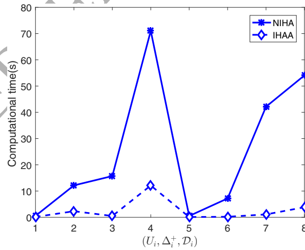
Figure 2: Average computational times using Algorithms 4.1 and 4.3 in \{(U_i, \Delta_i^+, \mathcal{D}_i) \mid 1 \leq i \leq 8\} .
