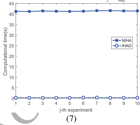
Figure 3: Computational times using Algorithms 4.1 and 4.5 in \{(U_i, \Delta_i^-, \mathcal{D}_i) \mid 1 \leq i \leq 8\} .
