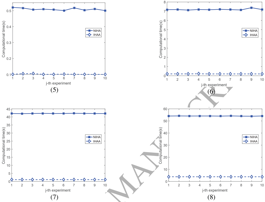
Figure 1: Computational times using Algorithms 4.1 and 4.3 in \{(U_i, \Delta_i^+, \mathcal{D}_i) \mid 1 \leq i \leq 8\} .
