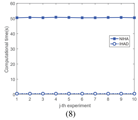
Figure 3: Computational times using Algorithms 4.1 and 4.5 in \{(U_i, \Delta_i^-, \mathcal{D}_i) \mid 1 \leq i \leq 8\} .
