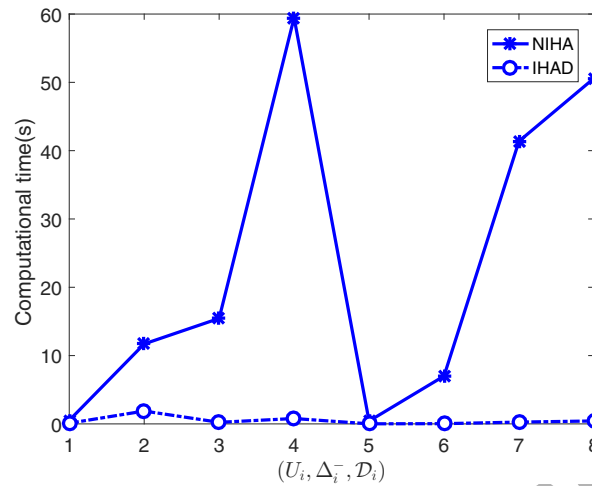
Figure 4: Average computational times using Algorithms 4.1 and 4.5 in \{(U_i, \Delta_i^-, \mathcal{D}_i) \mid 1 \leq i \leq 8\} .
