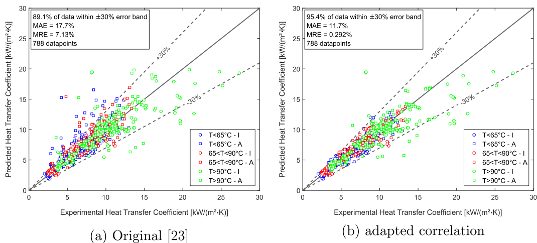
Fig. 9. Performance of the original and adapted version of the correlation of Choi et al. [23] for the combined dataset. (I = Intermittent flow; A = Annular flow).
