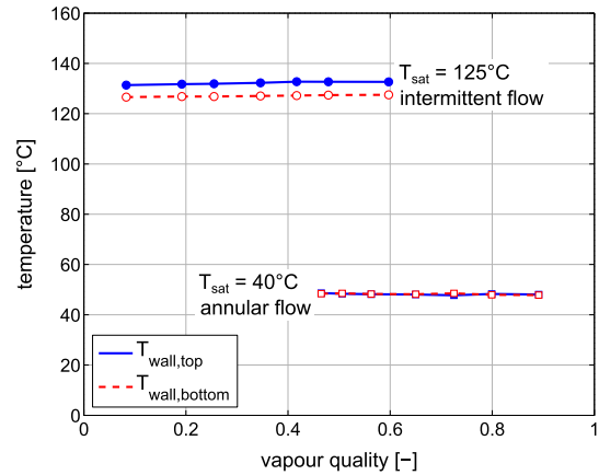
Fig. 3. The wall temperature measured at the top and bottom of the tube as a function of the vapour quality for different saturation temperatures. The heat flux at the wall is 54 kW/m 2 and the mass flux is 100 kg/(m 2 s). (circle = intermittent flow; square = annular flow).
