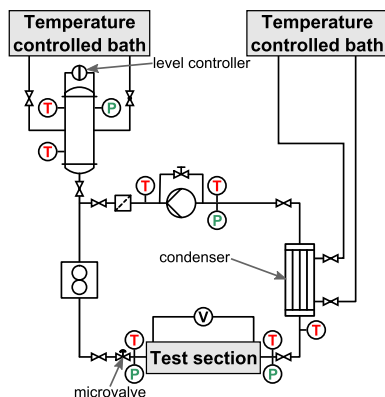
Fig. 1. A schematic representation of the experimental setup. (T = temperature measurement; P = pressure measurement).
