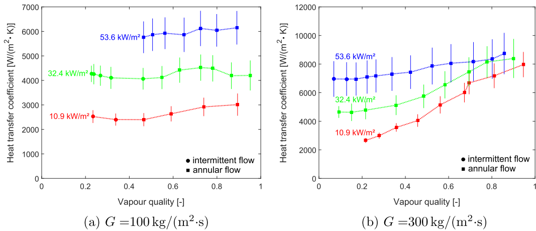
Fig. 5. The heat transfer coefficient as a function of the vapour quality for different heat fluxes at saturation temperature of 40 °C.
