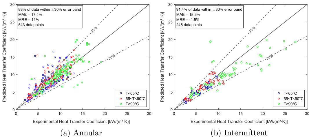
Fig. 8. Performance of the correlation of Choi et al. [23] for the combined dataset (dataset of Charnay et al. [14] and new experiments) for Annular and Intermittent flow.
