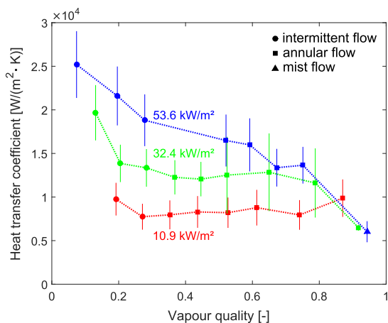
Fig. 6. The heat transfer coefficient as a function of the vapour quality for different heat fluxes at saturation temperature of 125 °C and a mass flux of 500 kg/(m 2 s).
