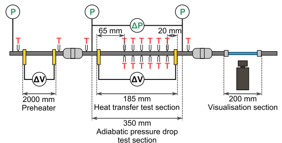
Fig. 2. A detailed schematic diagram of the test section. (T = temperature measurement; P = pressure measurement; \Delta V = DC power supply with voltage and current measurement).
