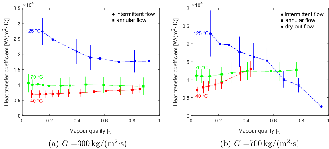
Fig. 4. The heat transfer coefficient as a function of the vapour quality for different saturation temperatures and a heat flux of 54 kW/m 2 .
