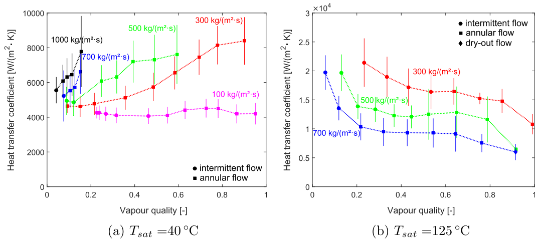
Fig. 7. The heat transfer coefficient as a function of the vapour quality for different mass fluxes and a heat flux of 32 kW/m 2 .
