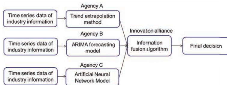
Fig. 4 Information fusion algorithm procedures.
