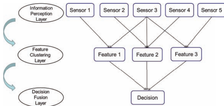
Fig. 2 Information fusion hierarchical structure model.
