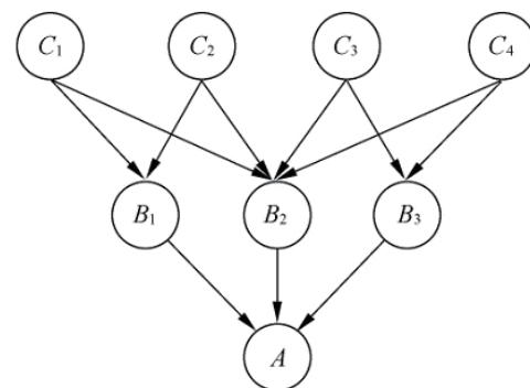
Fig. 1 Topological structure of a Bayesian network.
