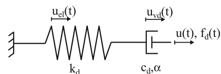
Fig. 1 Nonlinear viscous damper modeled with the Maxwell’s model
