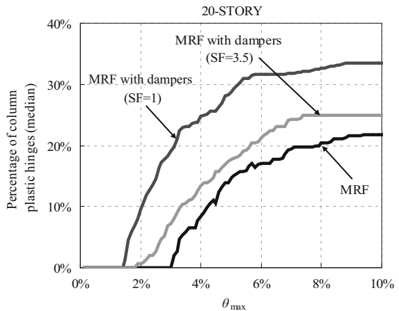
Fig. 8 Percentage of column plastic hinges in steel MRF, MRF with dampers (SF = 1) and MRF with viscous dampers (SF = 3.5). The figure refers to the 20-story building
