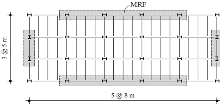
Fig. 1 Prototype building (plan view)
