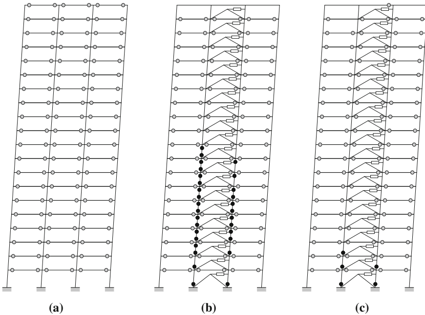
Fig. 9 Locations of plastic hinges in beams and columns at \theta_{max} equal to 2% under a specific ground motion for the 20-story a MRF; b MRF with dampers (SF = 1); and c MRF with dampers (SF = 3.5)
