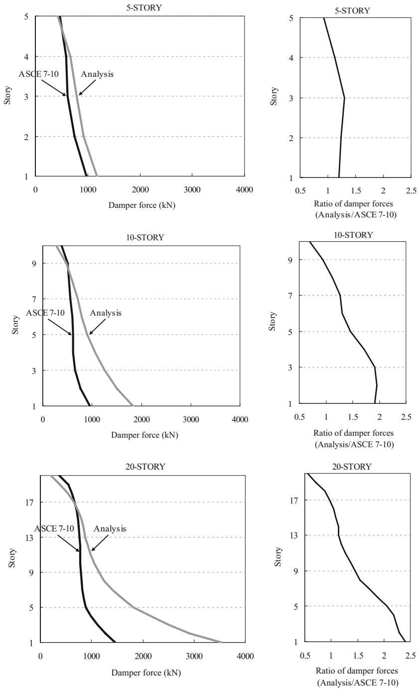
Fig. 6 Peak damper forces predicted by ASCE 7-10 and average peak damper forces from nonlinear dynamic analysis for 44 ground motions; both calculated for the DBE seismic intensity
