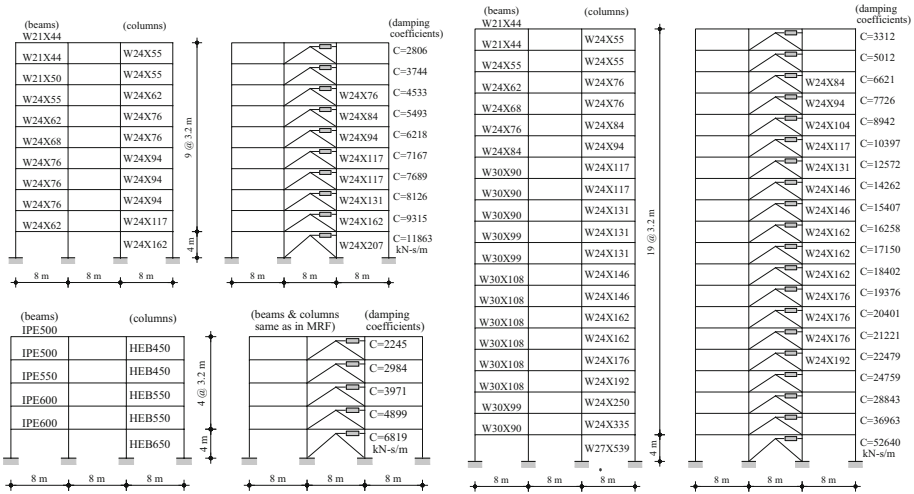
Fig. 2 Elevation view and beam/column cross-sections of the steel MRFs with and without viscous dampers. The damping coefficients of the viscous dampers are also provided. The beam/column cross-sections of the MRFs with viscous dampers are the same with those of the corresponding MRFs without dampers apart from the indicated interior columns
