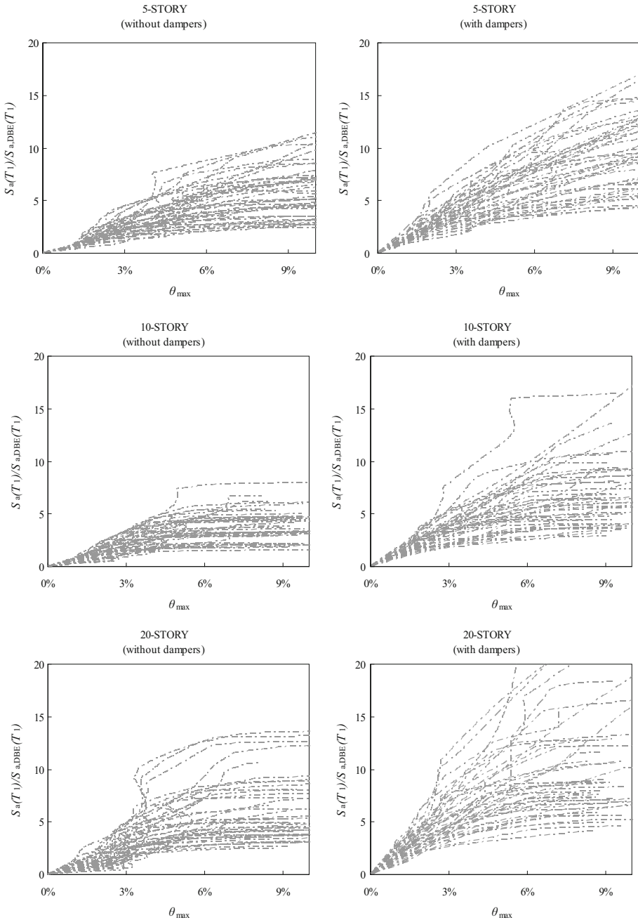
Fig. 4 IDA curves for the steel MRFs with and without viscous dampers
