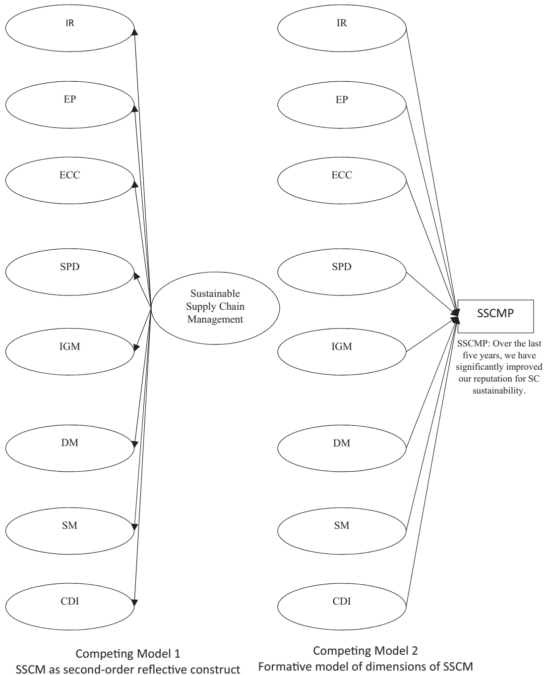
Fig. 3. Competing models.
