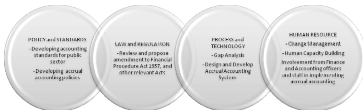
Fig. 1. Implementation Strategies.
