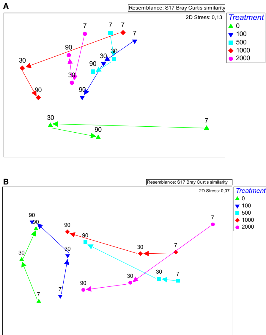
Fig. 3 Non-metric multidimensional scaling (NMDS) plot of fungal ( a ) and bacterial ( b ) community at different densities of C. fluminea (0, 100, 500, 1000 and 2000 ind. m -2 ) and sampling times (7, 30 and 90 days)
