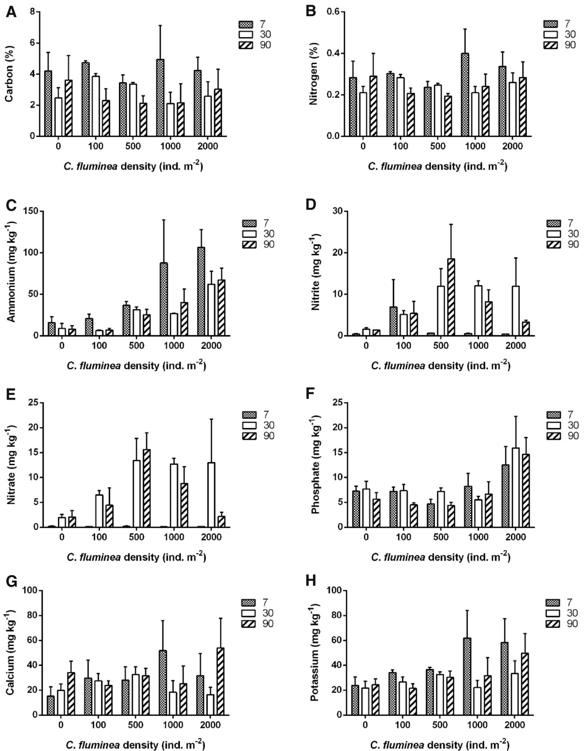
Fig. 1 Mean ( \pm SEM) values of organic C (a), total N (b) (%), \text{NH}_4^+ (c), \text{NO}_2^- (d), \text{NO}_3^- (e), \text{PO}_4^{3-} (f), Ca (g) and K (h) ( \text{mg kg}^{-1} ) at different densities of C. fluminea (0, 100, 500, 1000 and 2000 ind. m -2 ) and sampling times (7, 30 and 90 days)
