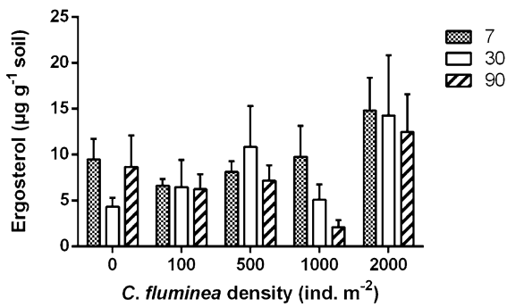
Fig. 2 Mean ( \pm SEM) values of ergosterol concentration ( \mu\text{g g}^{-1} soil) at different densities of C. fluminea (0, 100, 500, 1000 and 2000 ind. \text{m}^{-2} ) and sampling times (7, 30 and 90 days)
