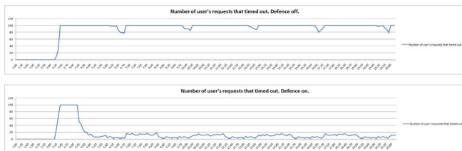
Fig. 6. The result of the simulation of the attack (the number of requests rejected by the timeout) without protection and using protection
