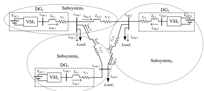
Fig. 1. Schematic diagram of an inverter interfaced microgrid.
