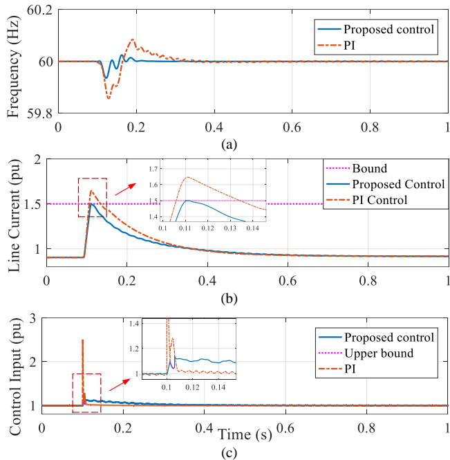
Fig. 5. Simulation results on the average model: (a). System frequency ( f ); (b). Line current ( i_{l,i} ). (c) Control signal ( v_{ad,i} ).
