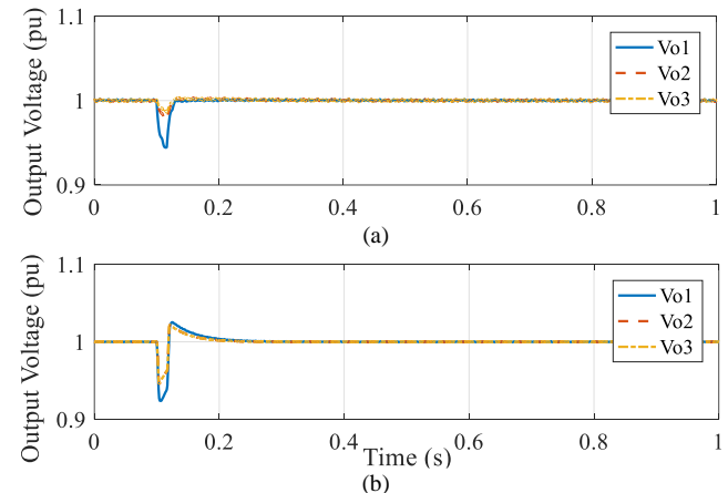
Fig. 8. Bus voltage responses on switching-level model: (a). PI controller; (b). Proposed controller.
