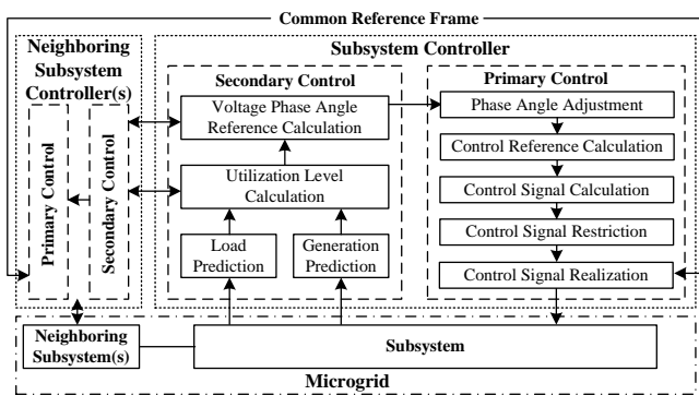
Fig. 2. The flowchart diagram of the proposed microgrid control scheme.
