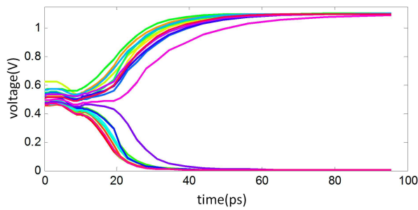
FIGURE 13: Monte Carlo simulation for the TSRAM PUF.
