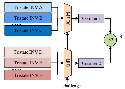
FIGURE 9: The proposed TCRO PUF.
