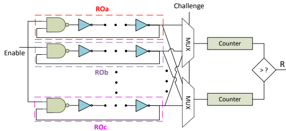
FIGURE 1: Conventional RO PUF by [2].
