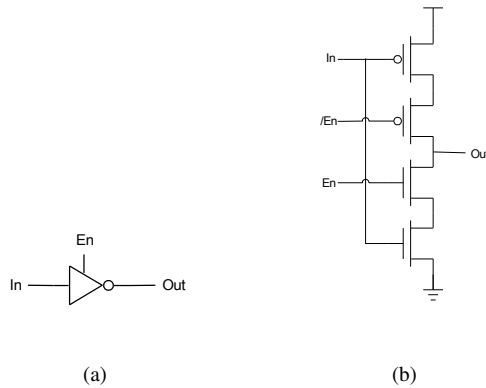
FIGURE 6: A tristate inverter. (a) Gate symbol. (b) Transistor level structure.
