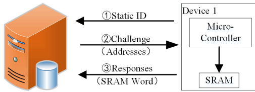
FIGURE 5: Typical protocol for SRAM PUF by [21].
