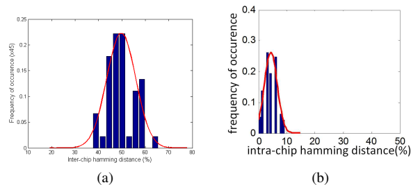
FIGURE 21: Hardware experimental results for the proposed TCRO PUF design. (a) Uniqueness. (b) Intra-chip HD.
