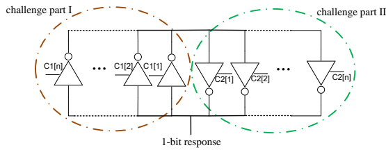
FIGURE 7: An 1-bit TSRAM PUF.
