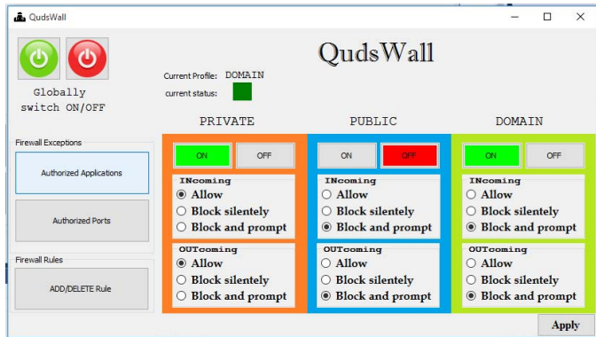
Fig. 6. QudsWall application Main Window.
