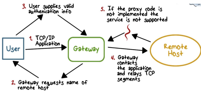
Fig. 4. Application-Gateway strategy
