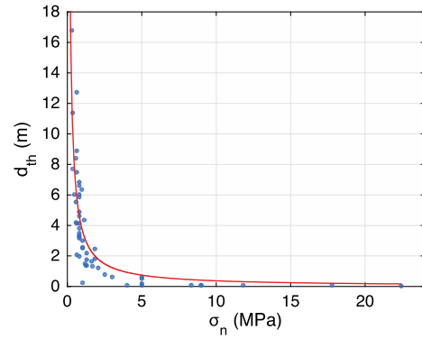
Fig. 3. The fit of d_{th} = 3.712 \|\sigma_n\|^{-1} (red line) compared with the laboratory experiments performed on clay material (see Table S5 in Supplementary Material for references). (For interpretation of the references to colour in this figure, the reader is referred to the web version of this article.)
