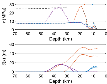
Fig. 10. Testing increased background initial stress outside of the asperity. a) The black dashed line is the yield strength. The dotted colour lines represent the initial shear stress where stress does not drop below the residual shear stress (i.e. \tau = \mu_d \sigma_n ). The x's are the nucleation locations for the new (i.e. dashed) set of simulations. b) The final slip distributions for each simulation where the colour and line type convention is same as the one used in subplot a). The solid lines are the slip distributions using the original initial stress distribution (see Fig. 4). (For interpretation of the references to colour in this figure, the reader is referred to the web version of this article.)
