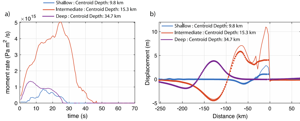
Fig. 6. a) Moment release rate with time. b) Vertical seafloor displacement (dotted lines) and estimated tsunami source (solid lines, details in Section A3 in Supplementary Information). Horizontal distance as in Fig. 2 where 0 km indicates the point where the fault reaches the seafloor. (For interpretation of the references to colour in this figure, the reader is referred to the web version of this article.)
