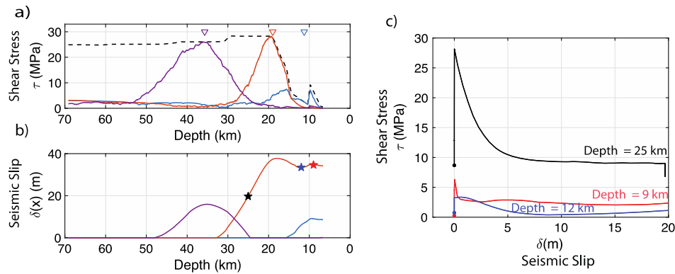
Fig. 4. Modelled environment earthquake source parameters. a) The different solid colours relate to the initial shear stress distributions used in the three simulations which reproduce a tsunamigenic great thrust earthquake (orange), tsunami earthquake (blue) and thrust earthquakes (purple). The same colour code is used for all subplots. Triangles are nucleation locations. Black dashed line is the fault strength. b) Slip distributions resulting from simulations where the colours relate to the initial stress distributions in a). c) Shear stress evolution with slip at three different depths (25 km black line, 12 km blue line, 9 km red line) taken from intermediate simulation (i.e., orange line in b). The locations are also highlighted by stars in subplot b) where a similar colour scale has been used. Dots denote the initial stress at each location. (For interpretation of the references to colour in this figure, the reader is referred to the web version of this article.)
