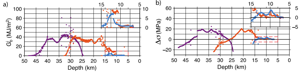
Fig. 5. a) Breakdown energy calculated at each point along the fault. Insets are expansions of the data inside the red dashed boxes. b) Static stress drop calculated at each point along the fault. (For interpretation of the references to colour in this figure, the reader is referred to the web version of this article.)
