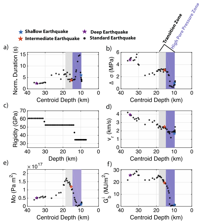
Fig. 7. Rupture parameters plotted against centroid depth for a number of simulations where only the location of the high stress asperity varies with depth. The purple box is the zone with very high pore pressure ( \lambda = 0.95 ); grey and purple boxes together demarcate the transition zone between clay-like and crystalline rock frictional parameters. a) Normalised earthquake duration; b) Average static stress drop; c) Shear modulus averaged across the fault plane to account of bi-material wall rocks; d) Average rupture velocity; e) Moment of the (1D) simulated earthquakes (details in Section A4 in Supplementary Material); and f) average breakdown energy. The stars indicate the three case studies presented in Fig. 2 with the same colour code applied. (For interpretation of the references to colour in this figure, the reader is referred to the web version of this article.)
