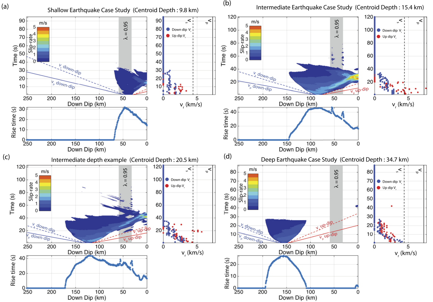
Fig. 8. Slip-rate, rupture velocity and rise-time observed in four simulations with increasing fault down-dip location of the asperity (40, 80, 120 and 160 km depth, respectively). These depths correspond to the hypocentral depths of the three cases presented in Fig. 2 and an additional great thrust earthquake which generated a down-dip travelling rupture pulse. In all subplots the solid and dashed lines are the P- and S-wave velocities in the oceanic material (i.e., yellow layer in Fig. 1) with the colour of the line indicating rupture direction (i.e. blue is to the left of the nucleation zone or down-dip, red is the right or up-dip). The light grey box behind the slip-rates defines the zone of very high pore pressure (i.e., \lambda = 0.95 ) in the wedge. a) Asperity in the wedge which corresponds to the shallow case study (blue line and dots in Figs. 2 and 3). b) Asperity at 20 km depth related to the intermediate case study (i.e., orange data in Figs. 2 and 3). c) Asperity at 27 km depth, an example of a great thrust earthquake with a down-dip travelling rupture pulse that was referred to in Section 3.4. d) Deep case study (i.e., 39 km) purple colour in Figs. 2 and 3. (For interpretation of the references to colour in this figure, the reader is referred to the web version of this article.)
