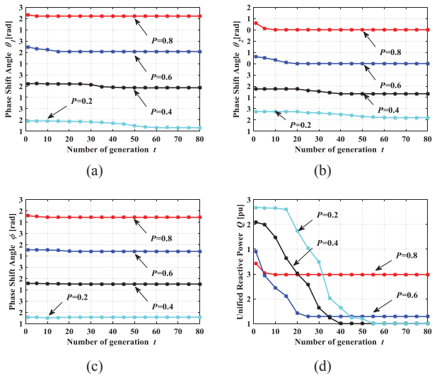
Fig. 8. (a) Phase shift \theta_1 varied with the number of iteration. (b) Phase shift \theta_2 varied with the number of iteration. (c) Phase shift \Phi varied with the number of iteration. (d) Reactive power Q varied with the number of iteration.
