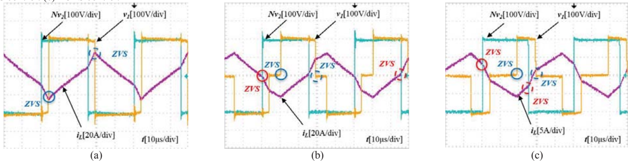
Fig. 22. Experiment waveforms for the reverse, buck mode and heavy-load condition: V_{in}=200V , V_{out}=200V and P=1200W . (a)SPS control.(b)EPS control.(c)POPS control.
