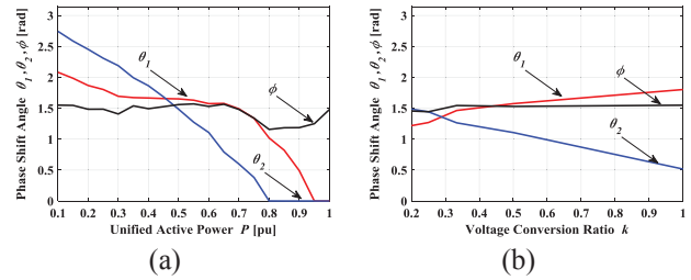
Fig. 14. (a) Phase shift variations with the unified active power under boost mode. (b) Phase shift variations with voltage conversion ratio k under boost mode.
