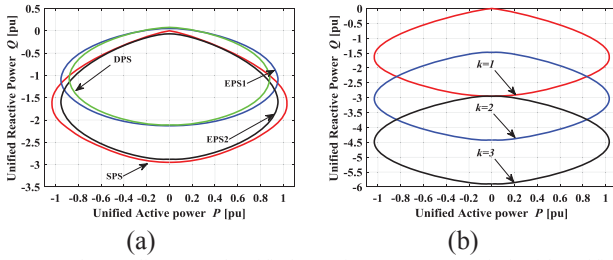
Fig.5. (a) Phasor diagram of unified reactive power Q varied with unified active power P using different control methods when k=1 . (b) Phasor diagram of unified reactive power Q varied with unified active power P under different voltage conversion ratio.
