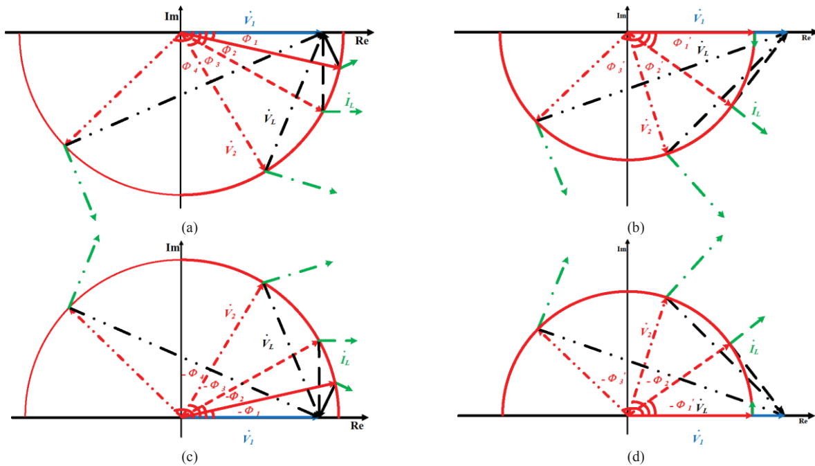
Fig.3. (a)Phasor diagram for the DAB when V_1 is leading V_2 and |V_1| < |V_2| . (b)Phasor diagram for the DAB when V_1 is leading V_2 and |V_1| > |V_2| . (c)Phasor diagram for the DAB when V_1 is lagging V_2 and |V_1| < |V_2| . (d)Phasor diagram for the DAB when V_1 is lagging V_2 and |V_1| > |V_2| .
