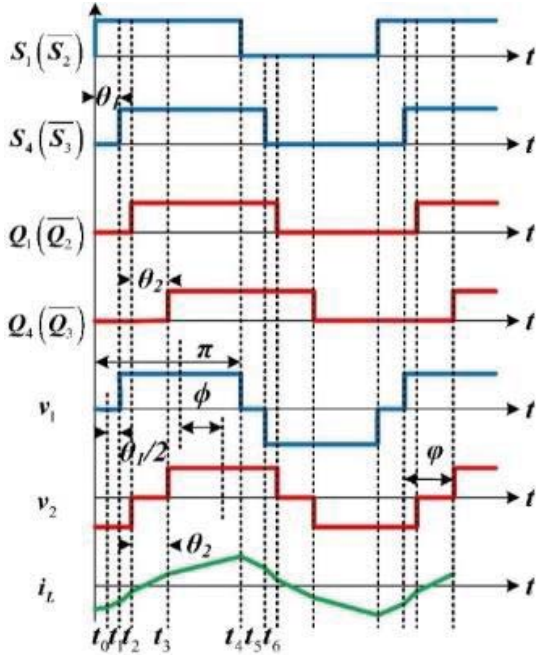
Fig. 2 Typical waveforms with the 3-level modulated phase shift method
