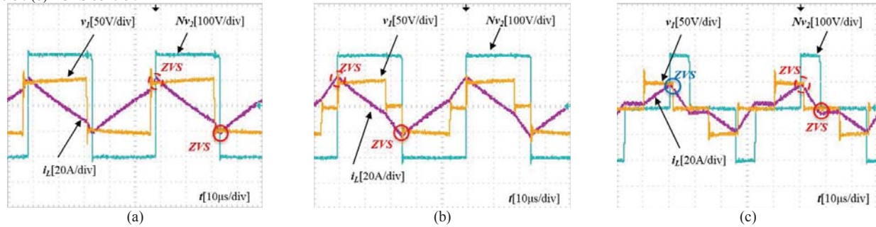
Fig. 24. Experiment waveforms for the forward, boost mode and light-load condition: V_{in}=50V , V_{out}=200V and P=150W . (a) SPS control. (b) EPS control. (c) POPS control.
