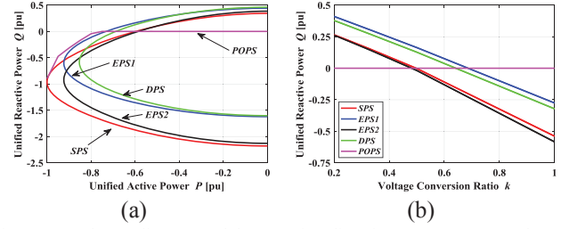
Fig. 13. (a) Phasor diagrams of the negative direction apparent power for different control method when k=1/2 . (b) Reactive power of different control method when P=0.6 varied with voltage conversion ratio k .
