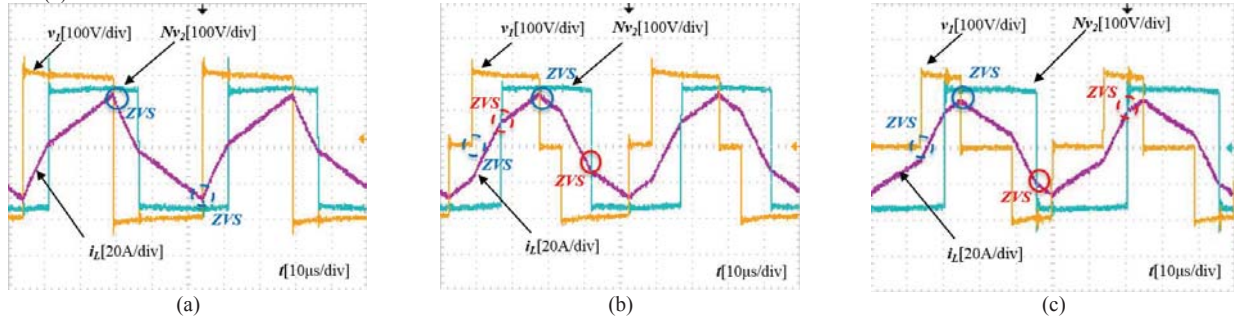
Fig. 21. Experiment waveform for the forward, buck mode (larger k ) and heavy-load condition: V_{in}=200V , V_{out}=160V and P=1200W . (a) SPS control.(b) EPS control.(c) POPS control.
