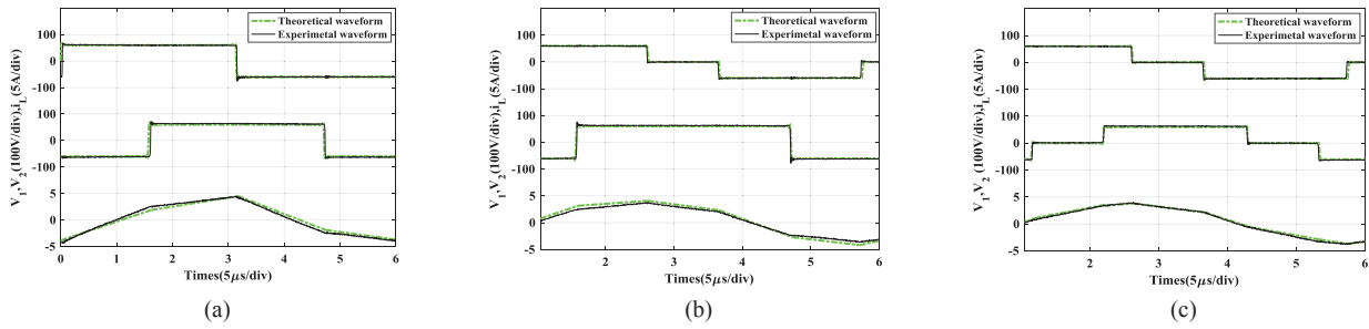
Fig. 18. Comparison of the theoretical and experimental waveforms under different control methods: (a) SPS. (b)EPS. (c)DPS.
