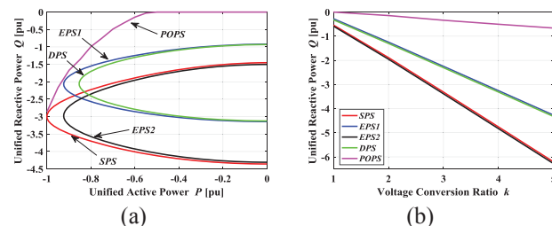
Fig. 10. (a) Phasor diagrams of the negative direction apparent power for different control method when k=2 . (b) Reactive power of different control method when P=-0.6 varied with voltage conversion ratio k .
