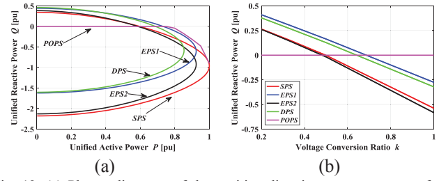
Fig. 12. (a) Phasor diagrams of the positive direction apparent power for different control method when k=1/2 . (b) Reactive power of different control method when P=0.4 varied with voltage conversion ratio k .
