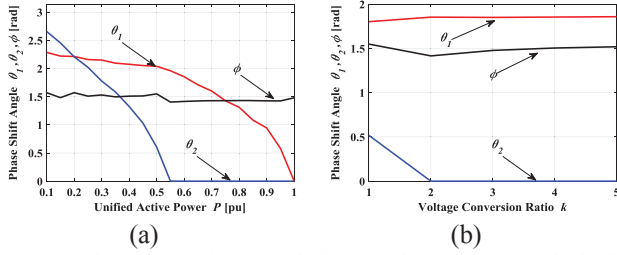
Fig. 11. (a) Phase shift variations with the unified active power under buck mode. (b) Phase shift variations with voltage conversion ratio k under buck mode.
