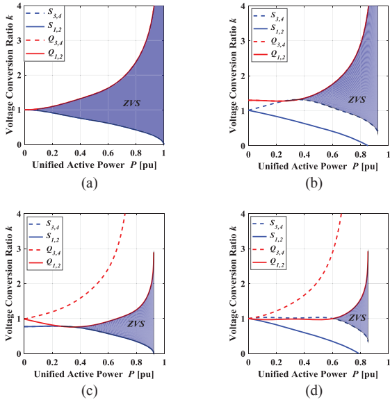
Fig. 15. (a) ZVS region for \theta_1=0, \theta_2=0 under SPS control. (b) ZVS region for \theta_1=\pi/4, \theta_2=0 under EPS1 control. (c) ZVS region for \theta_1=0, \theta_2=\pi/4 under EPS2 control. (d) ZVS region for \theta_1=\pi/4, \theta_2=\pi/4 under DPS control.
