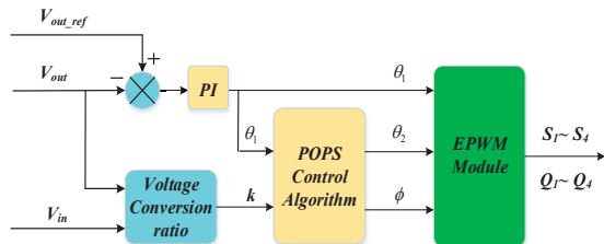
Fig. 17 Control implementation of the POPS algorithm.
