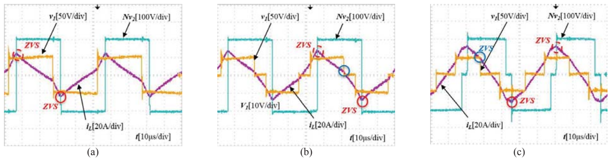
Fig. 23. Experiment waveforms for the forward, boost mode and heavy-load condition: V_{in}=50V , V_{out}=200V and P=300W . (a) SPS control. (b) EPS control. (c) POPS control.
