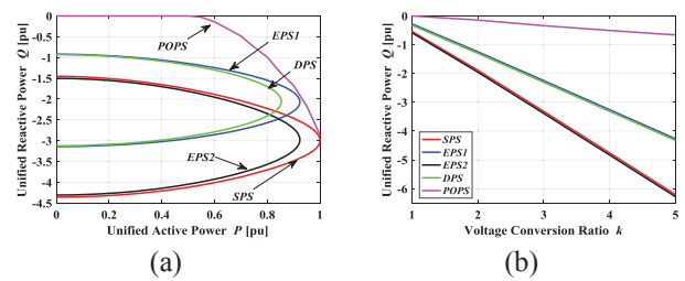
Fig. 9. (a) Phasor diagrams of the positive direction apparent power for different control method when k=2 . (b) Reactive power of different control method when P=0.6 varied with voltage conversion ratio k .
