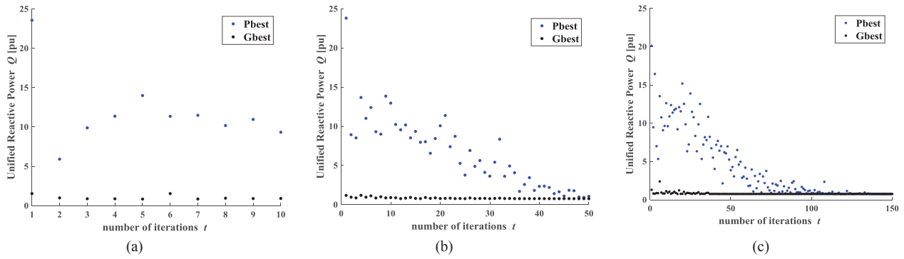
Fig. 7. (a) P_{best} and G_{best} of the unified reactive power Q varied with number of iteration when t_{max}=10 . (b) P_{best} and G_{best} of the unified reactive power Q varied with number of iteration when t_{max}=50 . (c) P_{best} and G_{best} of the unified reactive power Q varied with number of iteration when t_{max}=150 .
