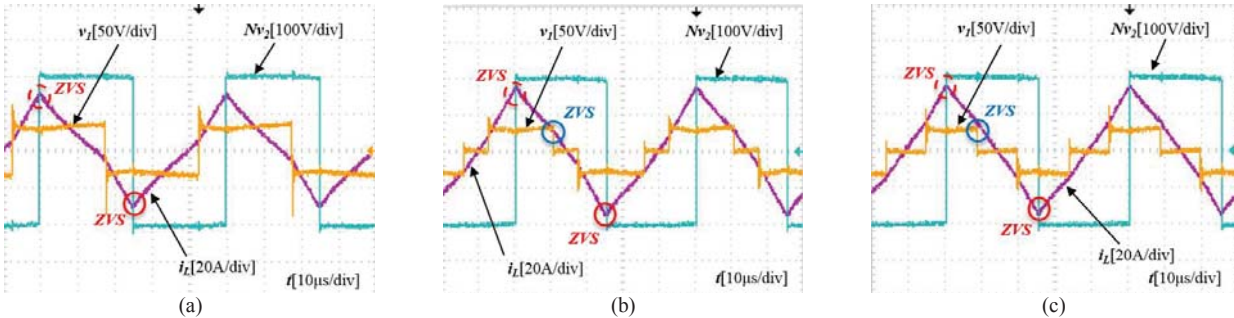
Fig. 25. Experiment waveforms for the forward, boost mode (smaller k ) and heavy-load condition: V_{in}=33.3V , V_{out}=200V and P=300W . (a) SPS control. (b) EPS control. (c) POPS control.
