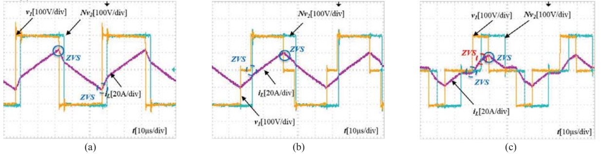
Fig. 20. Experimental waveforms for the forward, buck mode and light-load condition: V_{in}=200V , V_{out}=200V and P=600W . (a) SPS control.(b) EPS control.(c) POPS control.
