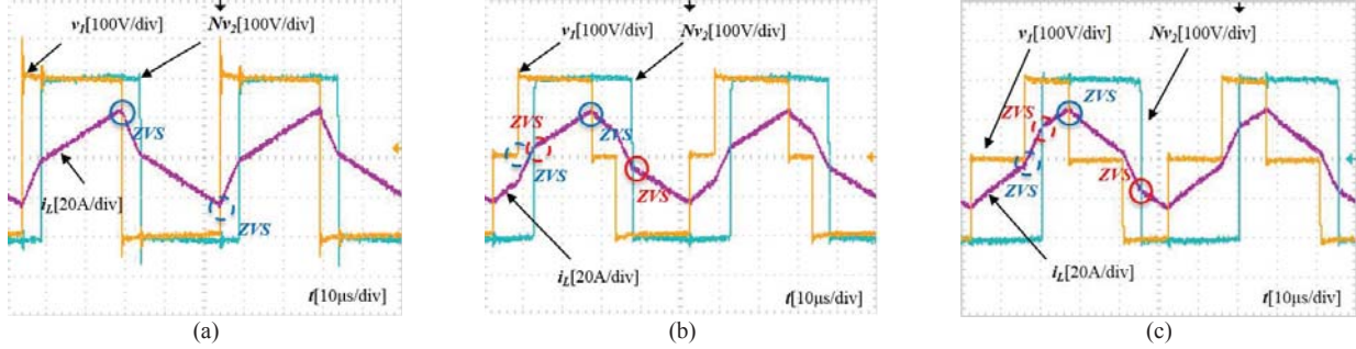
Fig. 19. Experimental waveforms for the forward, buck mode and heavy-load condition: V_{in}=200V , V_{out}=200V and P=1200W . (a) SPS control.(b) EPS control.(c) POPS control
