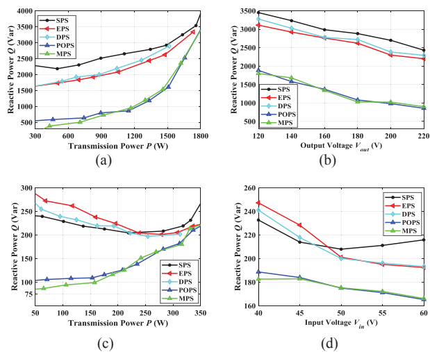
Fig. 26. (a) Reactive Power Q under various control methods varied with transmission power P when V_{in}=200V , V_{out}=200V . (b) Reactive Power Q varied with output voltage V_{out} when P=1200W , V_{in}=200V . (c) Reactive Power Q under various control methods varied with transmission power P when V_{in}=50V , V_{out}=200V . (d) Reactive Power Q varied with input voltage V_{in} when P=300W , V_{out}=200V .
