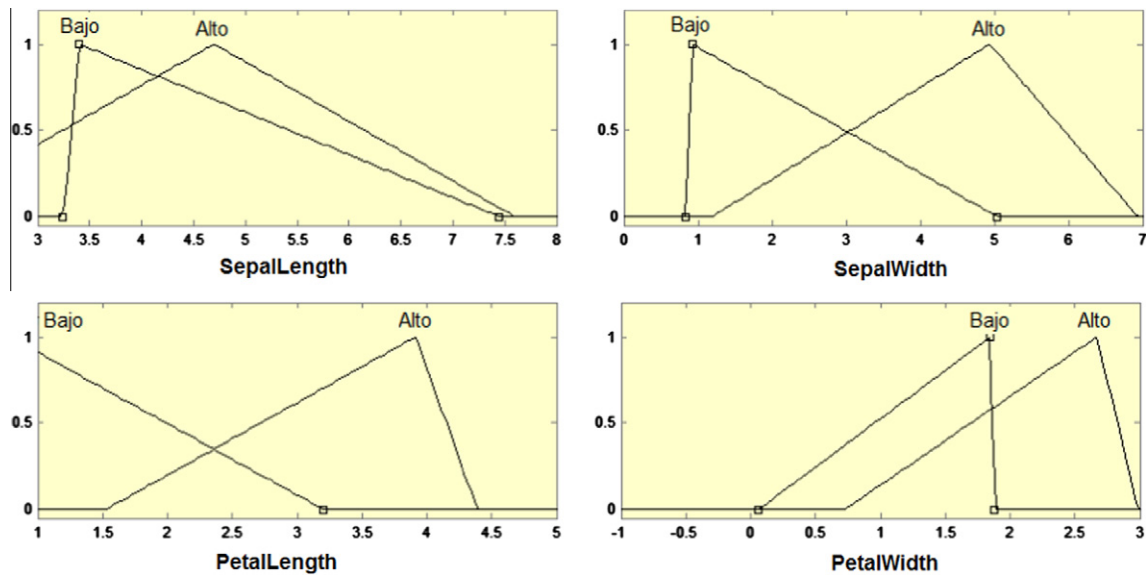
Fig. 21. Optimized membership functions of the fuzzy classifier.
