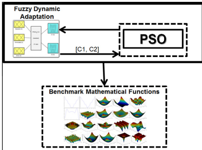
Fig. 13. Proposal for fuzzy dynamic adaptation of PSO.
