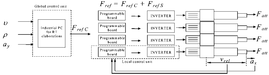
Figure 3. Scheme of the experimental set-up of the test vehicle for tangent and curved tests.
