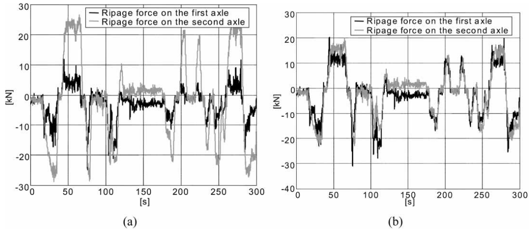
Figure 12. Time history of the ripage forces on the first and second axes of the vehicle with traditional (a) and 'virtually' controlled (b) yaw dampers (law pass filtered, f_{\text{cut}} = 10 Hz).
