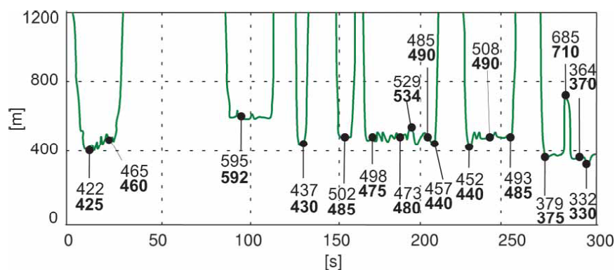
Figure 11. Time history of the estimated curve radius; comparison between some estimated (normal) and corresponding tabulated (bold) curve radius values.
