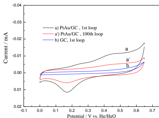
Figure 1. a) The 1 st and a') the 100 th CV loops of PtAu coating pulse electrodeposited on GC electrodes from a bath containing HAuCl 4 of 10 mmol/L, H 2 Pt Cl 6 of 10 mmol/L and H 2 SO 4 of 0.5mol/L at peak current density of 150 mA/cm 2 , pulse width of 10% and frequency of 100Hz, and b) the first CV loop of GC electrodes in O 2 -saturated 1 mol/L KOH solution
