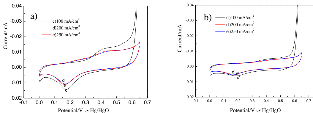
Figure 2. In O 2 -saturated 1 mol/L KOH solution a) the 1 st and b)the 100 th CV loops of PtAu coatings pulse electrodeposited from a bath containing HAuCl 4 of 10 mmol/L, H 2 Pt Cl 6 of 10 mmol/L and H 2 SO 4 of 0.5mol/L at different peak current densities, pulse width of 10% and frequency of 100Hz.
