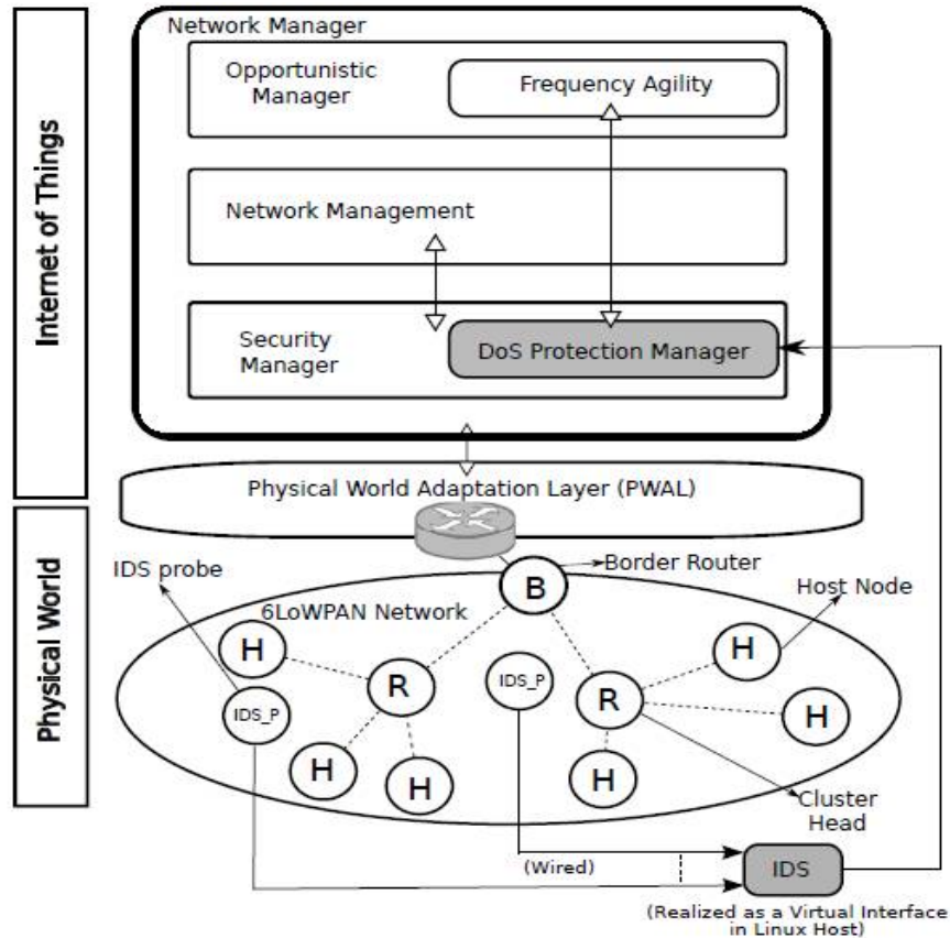
Figure No. 1 DoS Detection Architecture
