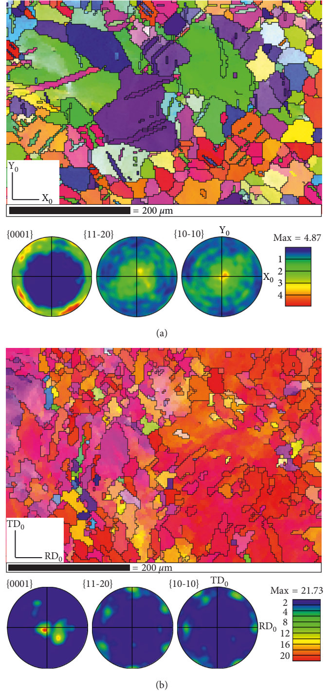
FIGURE 4: EBSD inverse pole figure (IPF) maps (top) and pole figures (bottom) showing microstructure and texture of the (a) cylindrical extruded bar and (b) rolled plate of the pure magnesium. The IPF maps reflect the orientations of the bar's extrusion direction (ED 0 ) and rolled plate's normal direction (ND 0 ) with respect to the local crystal frames. The measured pole figures show the initial texture of the processed (extruded and rolled) material. The reference frames (X 0 , Y 0 , ED 0 ) and (RD 0 , TD 0 , ND 0 ) are the same as in Figure 1.
