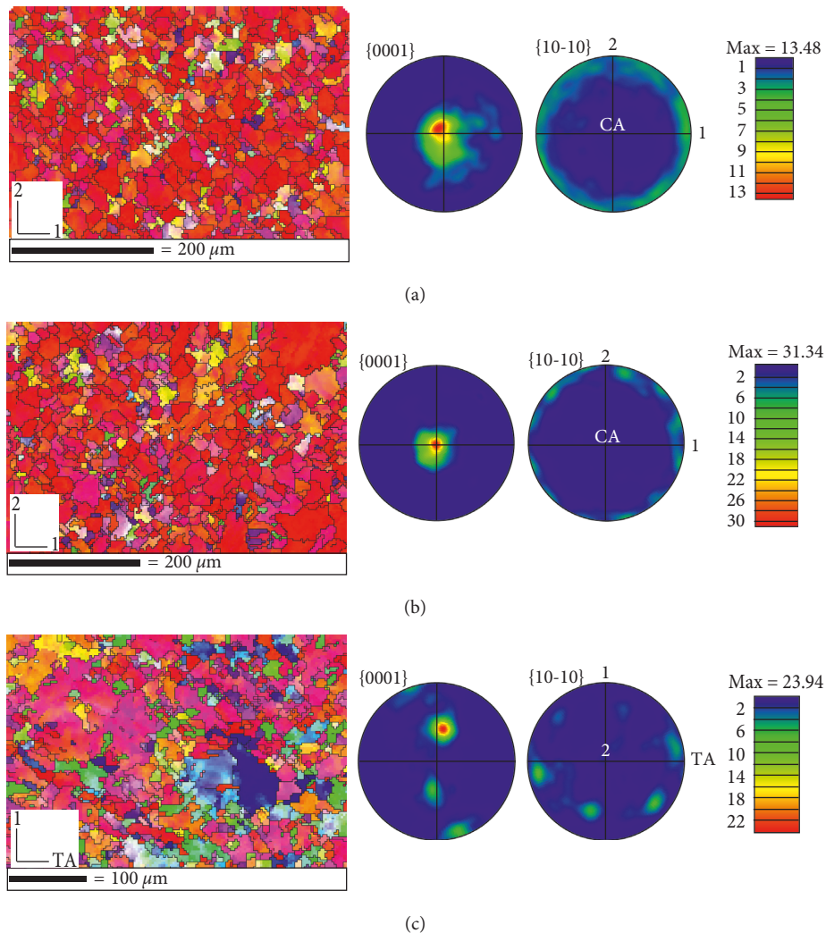
FIGURE 7: EBSD inverse pole figure (IPF) maps (left) and pole figures (right) showing texture of (a) CA0ED 0 and (b) CA0ND 0 pure magnesium samples after simple compression collected in a plane normal to the compression axis CA. The IPF and pole figures in (c) illustrate the texture of r sample after uniaxial tensile test collected in the tensile plane. The labels 1 and 2 in (c) represent the lateral directions of the tension test. The color legend is the same as in Figure 4.
