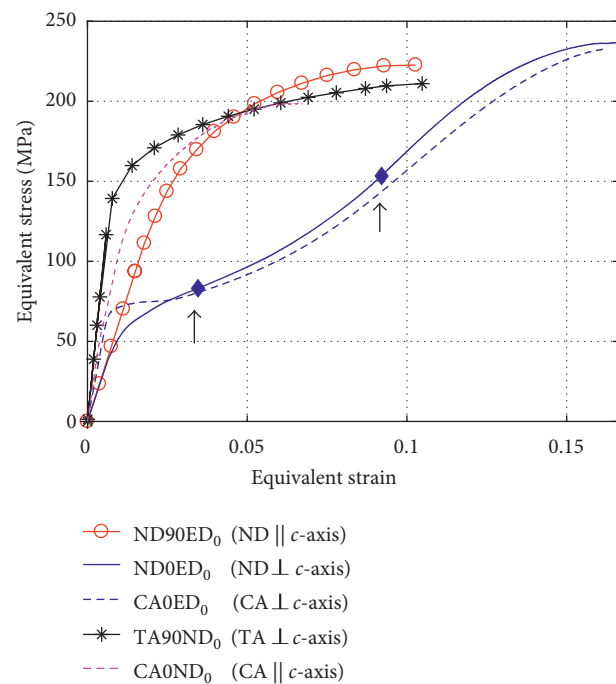
FIGURE 2: Flow curves of pure magnesium at room temperature under different mechanical tests including PSC (ND90ED 0 and ND0ED 0 ), simple compression (CA0ED 0 and CA0ND 0 ), and uniaxial tensile (TA90ND 0 ). The loading directions with respect to the typical crystallographic c -axis in most grains for each specimen are shown between parentheses.
