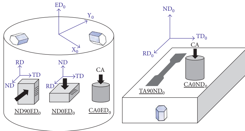
FIGURE 1: Schematic illustration of the orientations of the samples machined from the cylindrical extruded bar and rolled plate and used in plane strain compression (ND90ED 0 and ND0ED 0 ), simple compression (CA0ED 0 and CA0ND 0 ), and uniaxial tensile (TA90ND 0 ) tests. The typical crystallographic orientations of the c -axis resulting from extrusion and rolling processes are also shown.
