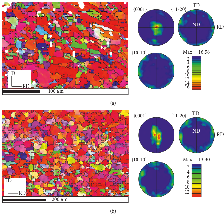
FIGURE 6: EBSD inverse pole figure (IPF) maps (left) and pole figures (right) showing microstructure and texture in RD-TD plane of the (a) ND0ED 0 and (b) ND90ED 0 pure magnesium samples after plane strain compression. The color legend is the same as in Figure 4.
