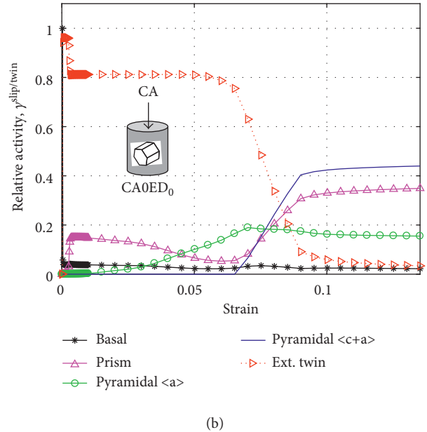
FIGURE 10: Relative slip and twin activities predicted by crystal plasticity simulation during simple compression of pure Mg for the two sample orientations tested in this study: (a) CA0ND 0 (CA \parallel c -axis) and (b) CA0ED 0 (CA \perp c -axis).
