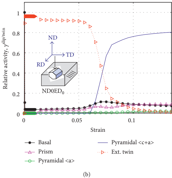
FIGURE 9: Relative slip and twin activities predicted by crystal plasticity simulation during plane strain compression of pure Mg for the two sample orientations tested in this study: (a) ND90ED 0 sample (ND \parallel c -axis) and (b) ND0ED 0 sample (ND \perp c -axis).
