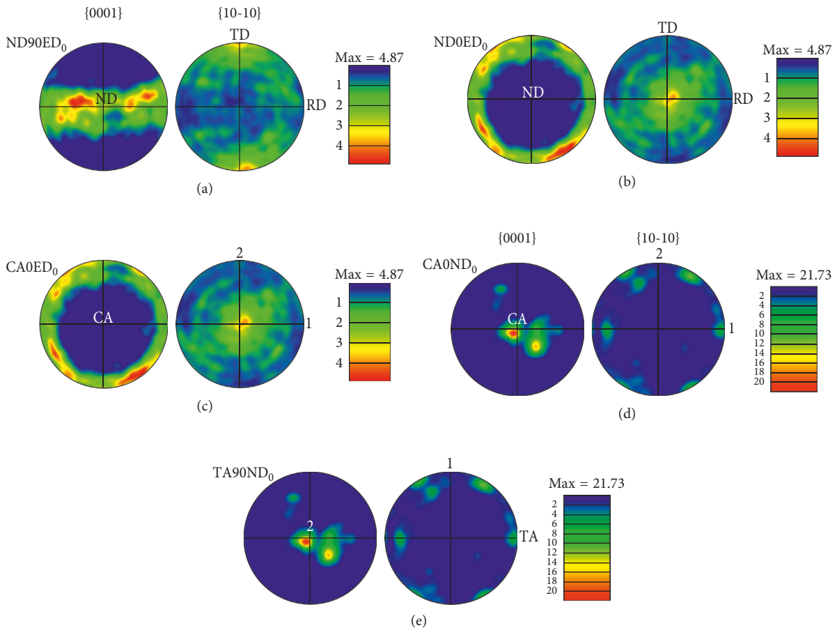
FIGURE 5: \{0001\} and \{10\bar{1}0\} pole figures of the initial texture for the five set of samples shown in Figure 1 using the reference frame for each mechanical test: (RD, TD, ND) for PSC, (1, 2, CA) for simple compression and (1, 2, TA) for uniaxial tension, where 1 and 2 refer to the lateral directions of the compression or tension test. The pole figures were obtained by appropriate rotations of the pole figures shown in Figure 4 with respect to the new reference frame. (a) ND90ED 0 . (b) ND0ED 0 . (c) CA0ED 0 . (d) CA0ND 0 . (e) TA90ND 0 .
