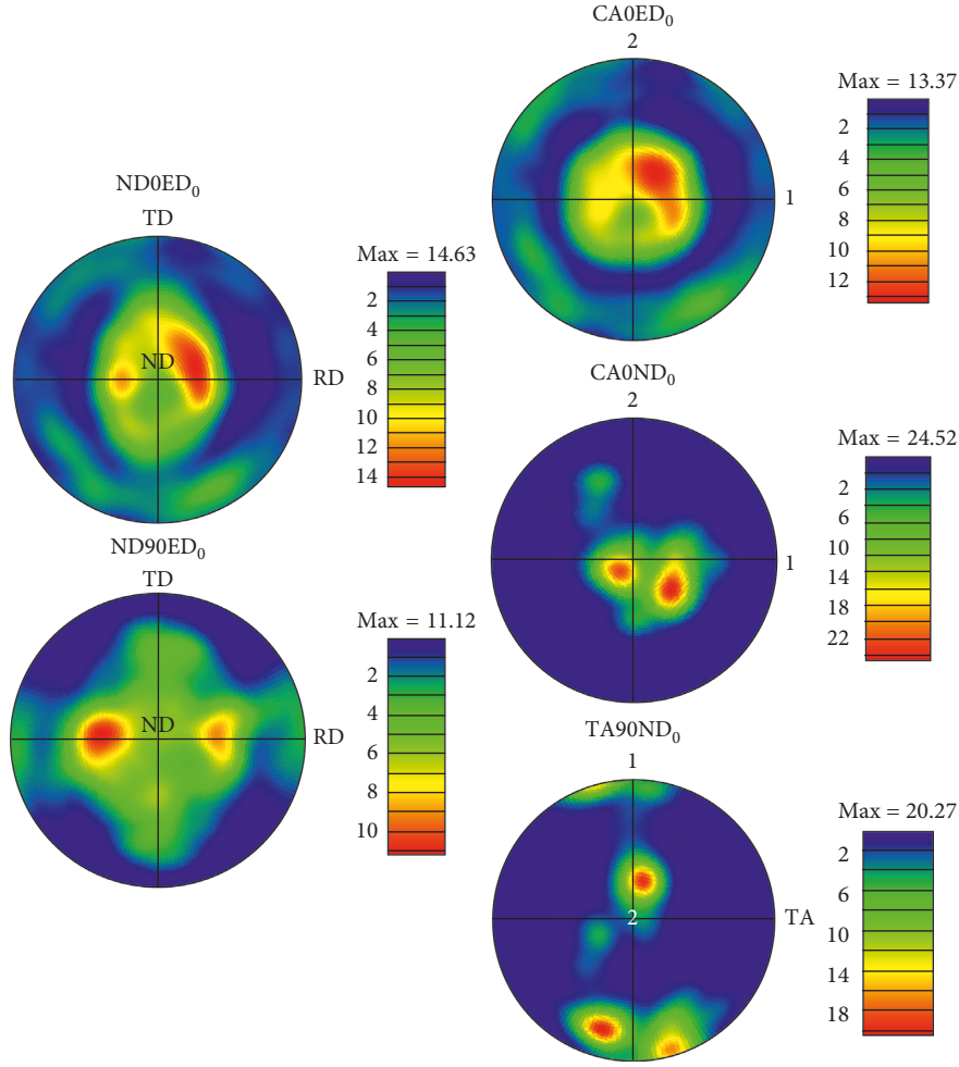
FIGURE 8: Predicted final texture ( \{0001\} pole figures) using crystal plasticity simulations under the five set of mechanical tests performed in this study: plane strain compression (ND0ED 0 and ND90ED 0 ), simple compression (CA0ED 0 and CA0ND 0 ), and uniaxial tension (TA90ND 0 ).
