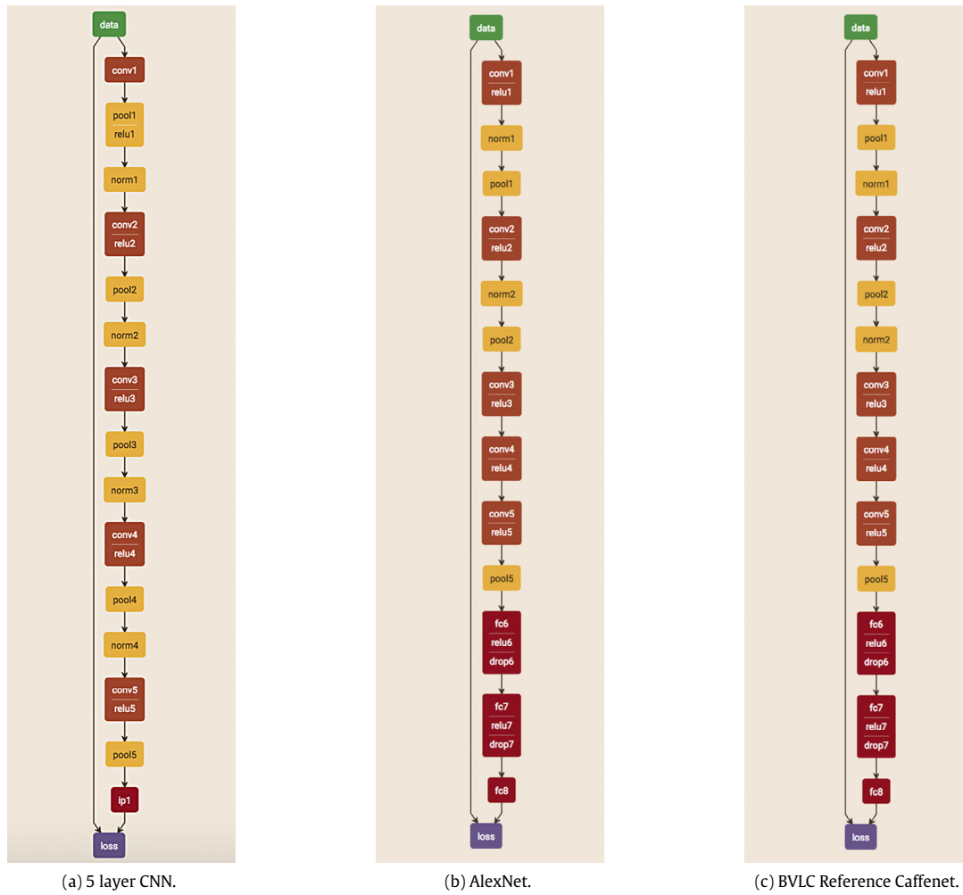
Fig. 1. Network architectures of various Convolutional Neural Networks used in our experiments. (Figures generated using Netscope Neural Network visualizer WWW5, 0000 .)
