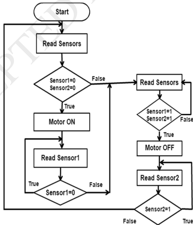
Figure 8. Flow chart of Web based Water Tank and Water Pump Control
