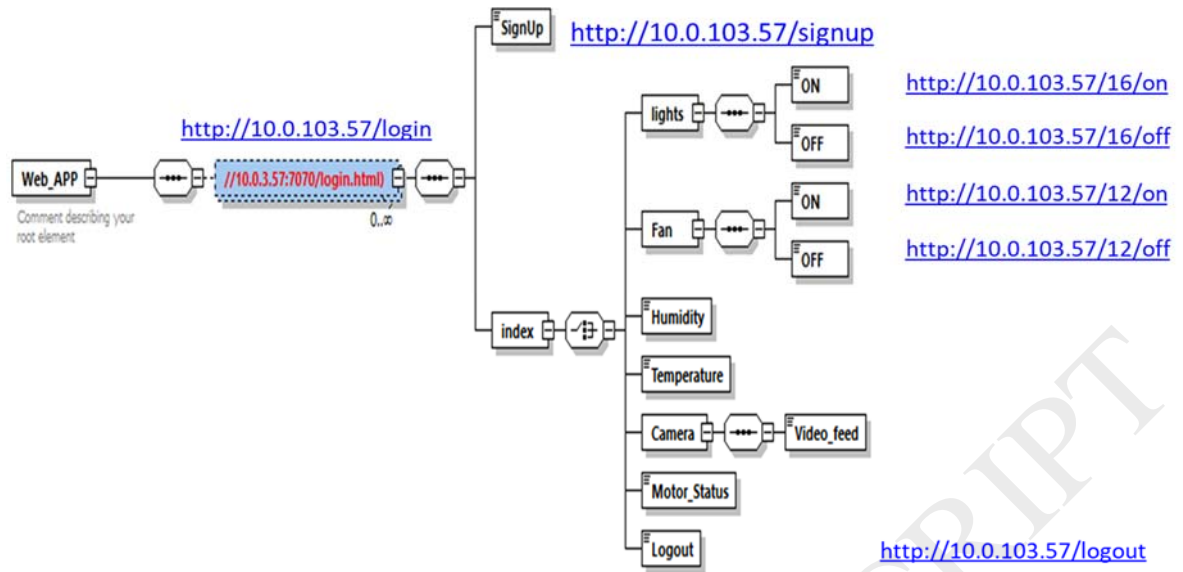
Figure 4. Overview of the RESTful Web URIs for the WoO based Smart Home Services
