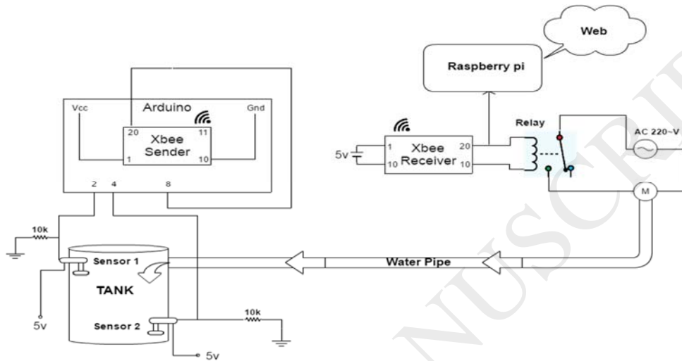
Figure 7. Web based Water Tank and Water Pump Control
