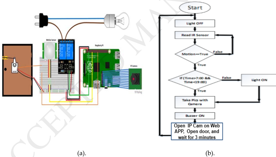
Figure 6. Web based door control using Raspberry PI camera as an IP camera, motion sensor and light control (a). Circuit diagram of web based door control (b). Flow chart of web based door control
