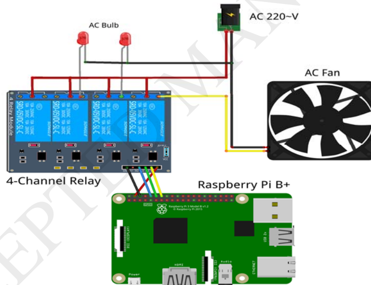
Figure 9. Circuit Diagram of WoO based lights and Fan Control
