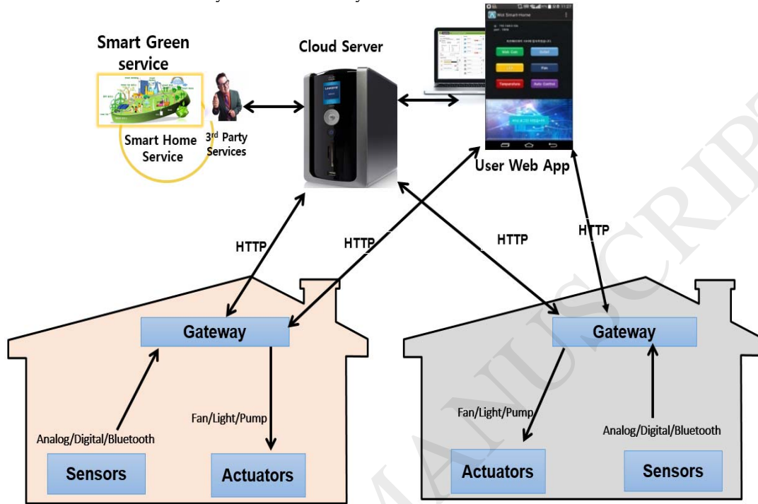
Figure 1. Conceptual Overview of Smart Home System Using Web-of-Objects and Cloud
