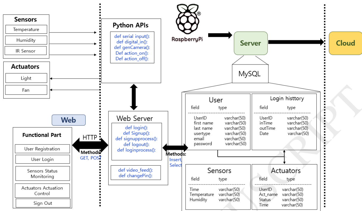
Figure 3. Detailed Architecture of Smart Home System Using Web-of-Objects and Cloud
