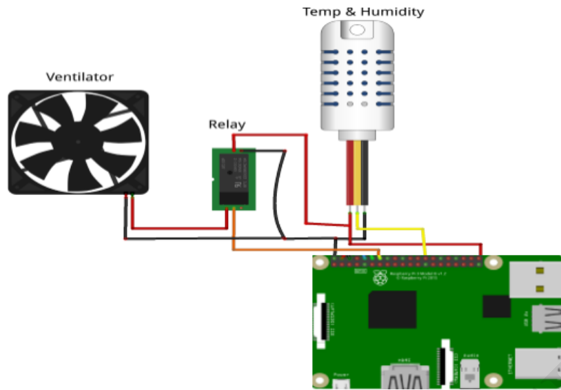
Figure 10. Circuit Diagram of WoO based Exhaust Fan Control using Humidity and Temperature Sensors
