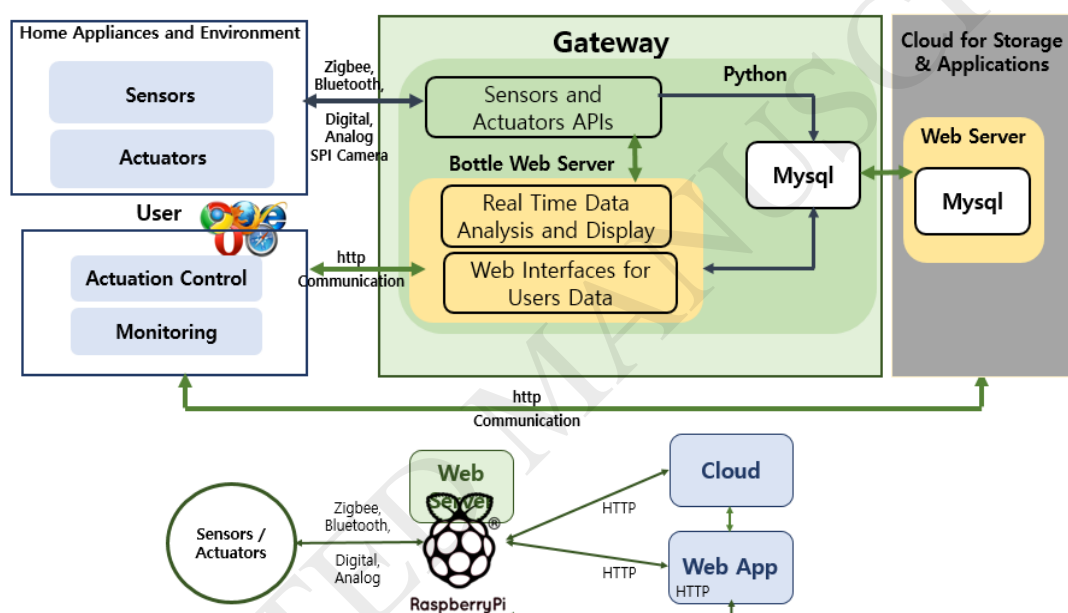
Figure 2. Proposed Architecture of Smart Home System Using Web-of-Objects and Cloud
