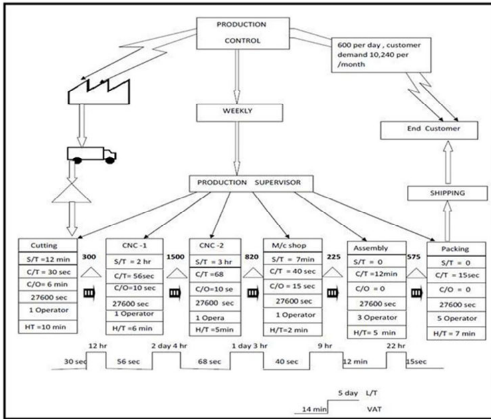
Figure 2 current state value stream mapping
