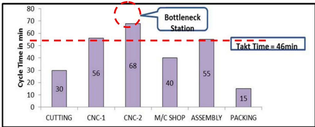
Figure 4: Bottleneck process
