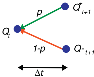
Fig. 2. Cox et al. binomial tree continuation calculus (1979). Source: Authors.
