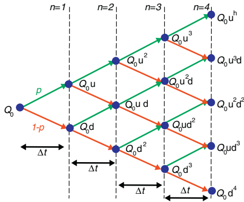
Fig. 1. Binomial tree of the Cox, Ross, and Rubinstein model (1979). Source: Authors.
