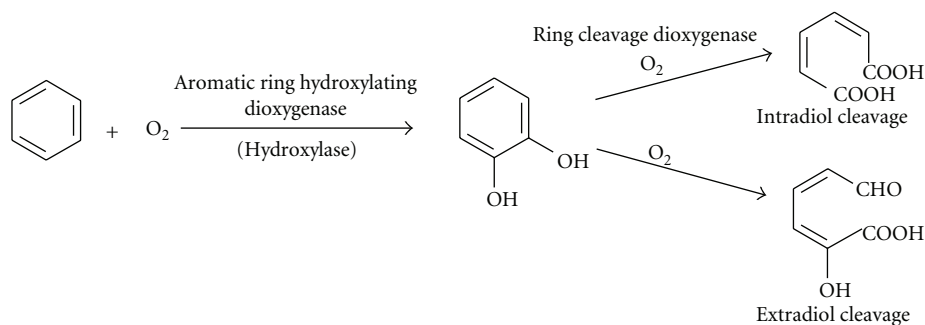
FIGURE 3: Degradation of aromatic compound by dioxygenase [17, 18].
